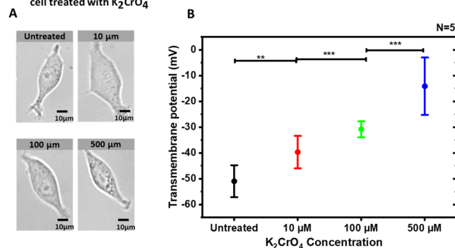
Figure 2. Dose–response effect of potassium chromate on the transmembrane potential of the HEK293H cells. (A) Bright-field microscope images (40X) of the HEK293H cells after 90 min K_2CrO_4 treatment with various concentrations. (B) Transmembrane potential of the HEK293H cells after the treatment of K_2CrO_4 with different concentrations. The average transmembrane potentials are untreated ( -50.9 \pm 2.48 mV), K_2CrO_4 [ 10 \mu M ] ( -39.6 \pm 2.5 mV), K_2CrO_4 [ 100 \mu M ] ( -30.8 \pm 1.2 mV), and K_2CrO_4 [ 500 \mu M ] ( -14.1 \pm 4.5 mV). For statistics with N = 5 : untreated vs 10 \mu M , “***” P < 0.01 ; 10 \mu M vs 100 \mu M , “***” P < 0.001 ; 100 \mu M vs 500 \mu M , “***” P < 0.001 . Both optical images and transmembrane potential measurements were taken about 90 min after the treatment.
