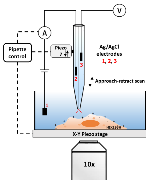
Figure 1. Scheme of P-SICM on simultaneous recording of the topography and surface potential of cell membrane. The nanopipette is mounted on a Z-piezo actuator. The ion current that flows between the Ag/AgCl electrodes 1 and 2 is used as the feedback signal to control the distance between the nanopipette tip and the cell surface. Electrode 3 in another barrel is connected to a high-impedance differential amplifier to measure the extracellular potential near the pipette tip.
