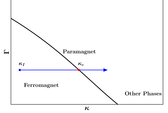
FIG. 1. Schematic representation of our quench protocol, superimposed on a schematic ground-state phase diagram of the ANNNI chain.
