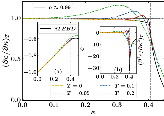
FIG. 9. Thermal equilibrium energy per site e and its derivatives at different T . The main panel shows (\partial e / \partial \kappa)_T , inset (a) shows e versus \kappa at constant temperature, and inset (b) shows (\partial^2 e / \partial \kappa^2)_T . Results are shown for different values of T (the main panel and the insets share the legend). The solid (black) curve ( T = 0 ) shows the iTEBD results for the ground state, while the other curves show NLCE results. Also depicted in the main panel is a = \langle \sigma_i^x \sigma_{i+2}^x \rangle_{\rho_I} / L \approx 0.99 for T_I \lesssim 0.1 . The vertical dashed lines mark the critical \kappa_c \approx 0.41 .
