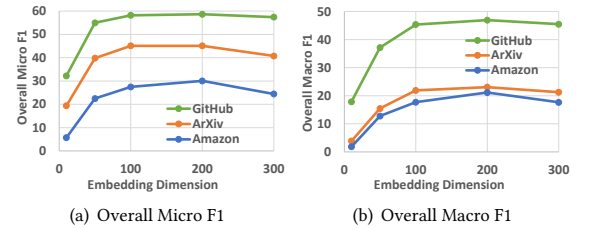
Figure 3: Performance of HiMECAT with different embedding dimensions ( p ).
