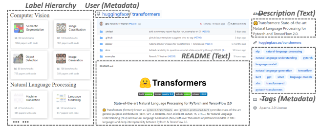
(a) GitHub Repository. Label Hierarchy: PaperWithCode Task Taxonomy ( https://paperswithcode.com/sota ); Text: Description and README; Metadata: User and Tag.
