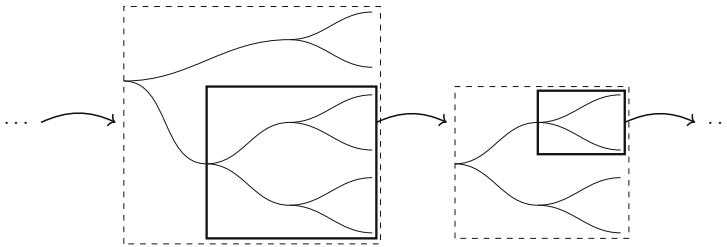
Fig. 2 Subsystem-recursivity in time shared by both many-worlds and pilot-wave theory
