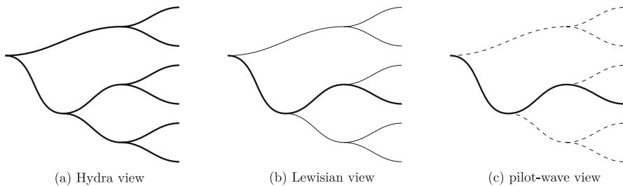
Fig. 3 Schematic illustrations of the many-worlds completions of a branching history algebra on the Hydra and Lewisian views, as well as a sketch of the Bohmian completion
