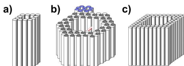
Fig. 8 Rigid DNA origami nanocages that provide nanoconfinement to the folding and unfolding of
