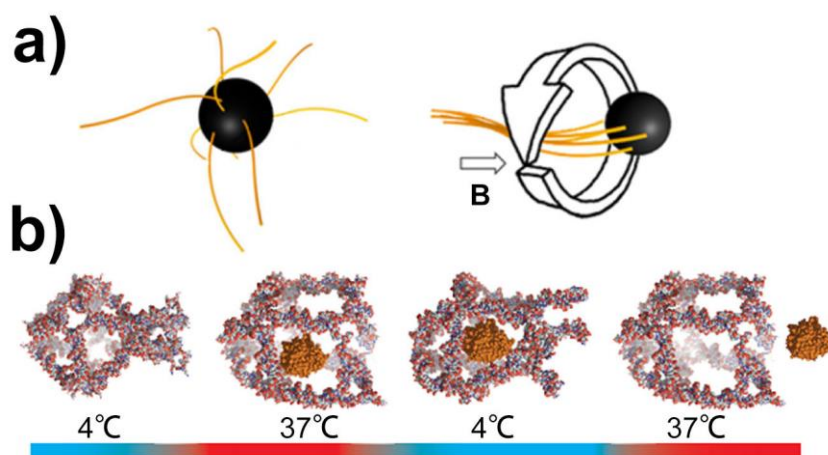
Fig. 10 Schematics of (a) magnetic beads modified with artificial flagella which move in an external magnetic field (B) 98 (reprinted with permission from Ref. 98, the direct link is https://pubs.acs.org/doi/10.1021/acs.nanolett.5b03716 and further permissions related to this material excerpted should be directed to the ACS) and (b) temperature-controlled morphological change of nanocages. From left to right, a contracted nanocage (4°C), a cargo containing nanocage (37°C), a packaged nanocage (4°C), and the nanocage with the released cargo (37°C) 100 (reprinted with permission from Ref. 100, Copyright (2013) American Chemical Society).
