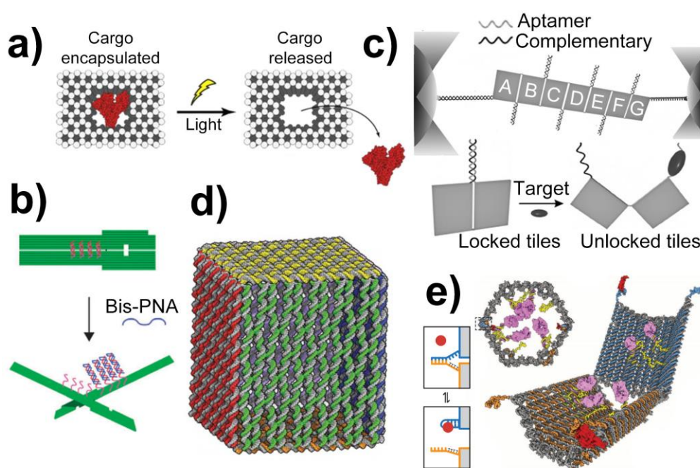
Fig. 11 Examples of localized plasticity in DNA origami nanoassemblies. (a) Light-sensitive
