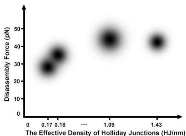
Fig. 15 Relationship between disassembly force (pN) of DNA origami nanoassemblies and densities of Holliday Junctions (HJ/nm) along the direction of applied force. This plot uses published data. 24
