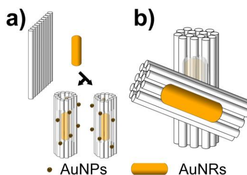
Fig. 9 Rigid DNA structures serving as templates for (a) a chiral plasma device 89 (reproduced from Ref. 89 with permission from John Wiley and Sons, copyright 2017) and (b) a biosensing device 90 (reproduced from Ref. 90 with permission from ACS, copyright 2018).
