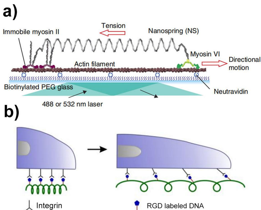
Fig. 7 DNA nanosprings. (a) A programmable nanospring is applied to myosin VI heads 5 (reprinted with permission from Springer Nature). (b) A pH sensitive DNA nanospring controls cell motions 74 (reprinted with permission from Ref. 74, Copyright (2021) American Chemical Society).
