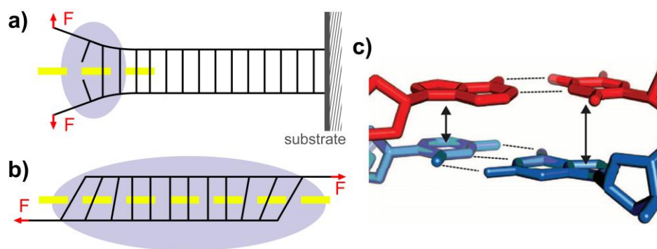
Fig. 2 Schematics of (a) unzipping of dsDNA, (b) shearing of dsDNA, and (c) stacking of two adjacent Watson-Crick base pairs. The arrows in (c) represent stacking interactions and the dashed lines represent hydrogen bonds 20 (reprinted with permission from AAAS).
