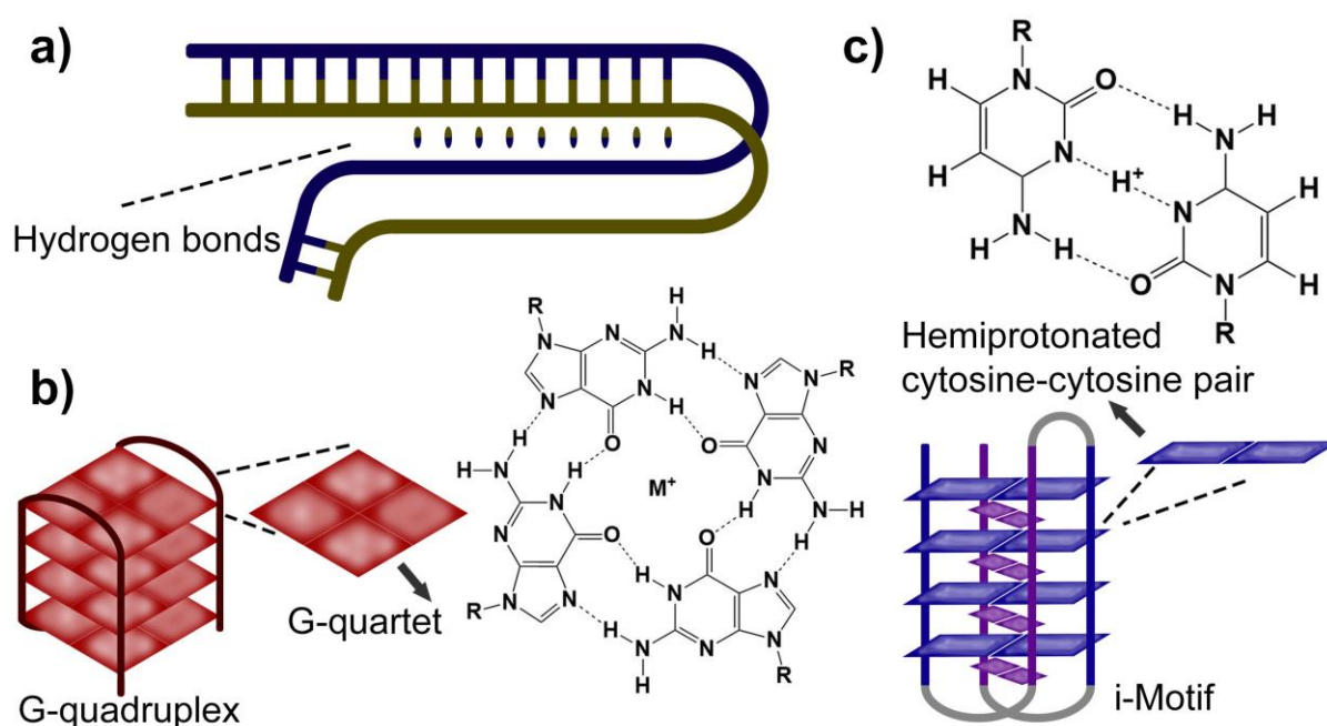
Fig. 4 DNA secondary structures. (a) a H-DNA structure (the oval links indicate Hoogsteen hydrogen bonds), (b) a G-quadruplex structure and (c) an i-Motif structure. The M^+ in the chemical structure in (b) refers to a monovalent ion such as Na^+ . 46,47
