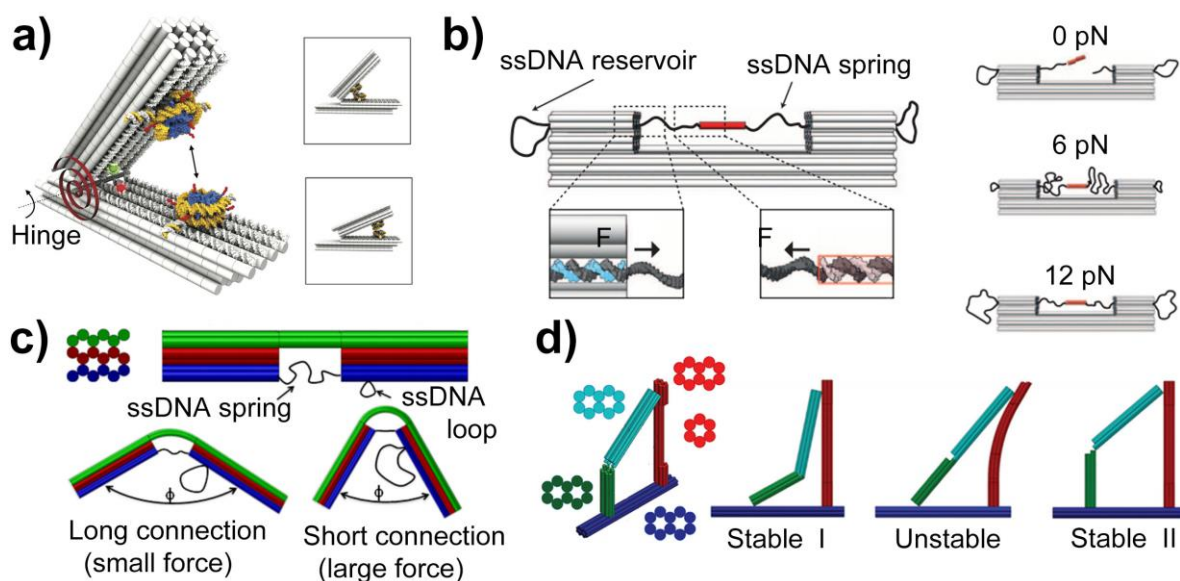
Fig. 6 DNA origami structures exploiting reversible elasticity properties. (a) A force spectrometer. The red cylinder represents the spring and hinge 8,67 (reprinted from Ref. 8 of AAAS). (b) Nanoclamps that maintain 0 pN, 6 pN, and 12 pN tension in ssDNA 71 (reprinted with permission from AAAS). (c) Adjustable DNA geometry components (Left: relaxed state; Right: tightened state) 72 (reprinted with permission from Ref. 72, Copyright (2014) American Chemical Society). (d) A bistable nanomechanism with three states 73 (reprinted with permission from Ref. 73, Copyright (2015) American Chemical Society). Circles to the left of (c) and (d) represent cross sections (helix bundles) of DNA origami backbones.
