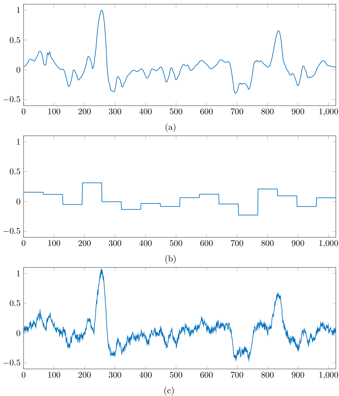
Figure 6. Experiment of section 5.2: (a) Original signal \bar{x} . (b) Piecewise constant approximation p_1 . (c) Recovered signal.
