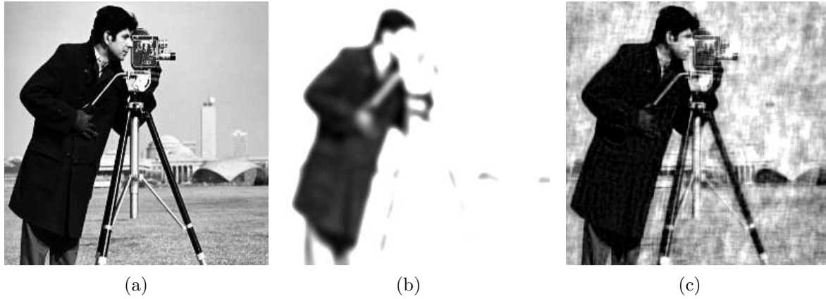
Figure 5. Experiment of section 5.1: (a) Original image \bar{x} . (b) Degraded image p_1 . (c) Recovered image.
