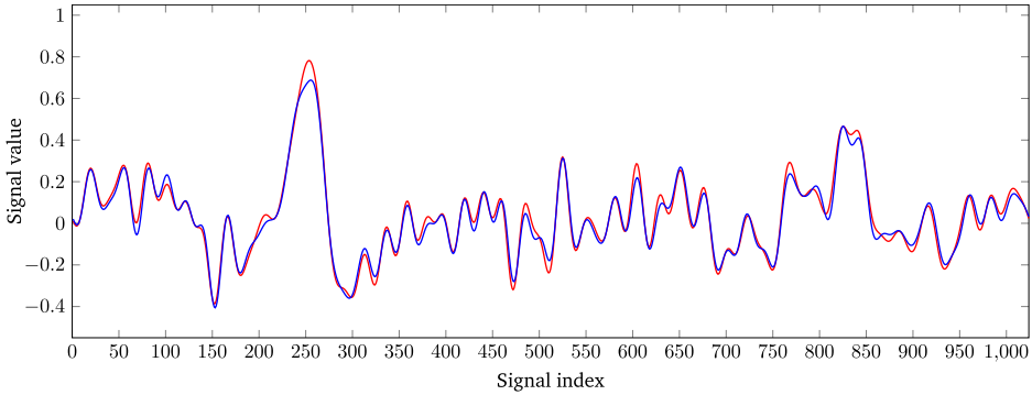
Fig. 3. Solution x_\infty (red) and the approximate recovery obtained with 1000 iterations of algorithm (4.3), which exploits affine constraints (blue). (For interpretation of the references to color in this figure legend, the reader is referred to the web version of this article.)
