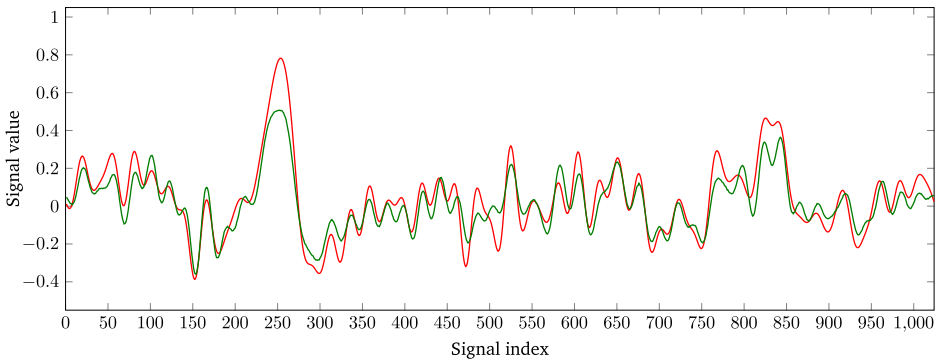
Fig. 4. Solution x_\infty (red) and the approximate recovery obtained with 1000 iterations of algorithm (4.5), which does not exploit affine constraints (green). (For interpretation of the references to color in this figure legend, the reader is referred to the web version of this article.)
