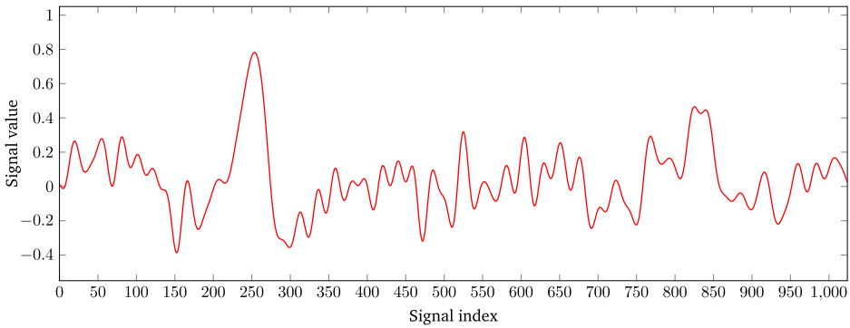
Fig. 2. Solution x_\infty to (5.1).
