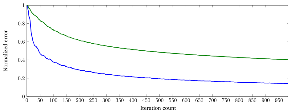
Fig. 5. Normalized error \|x_n - x_\infty\|/\|x_0 - x_\infty\| versus iteration count n \in \{0, \dots, 1000\} for algorithm (4.3) (blue) and algorithm (4.5) (green). (For interpretation of the references to color in this figure legend, the reader is referred to the web version of this article.)
