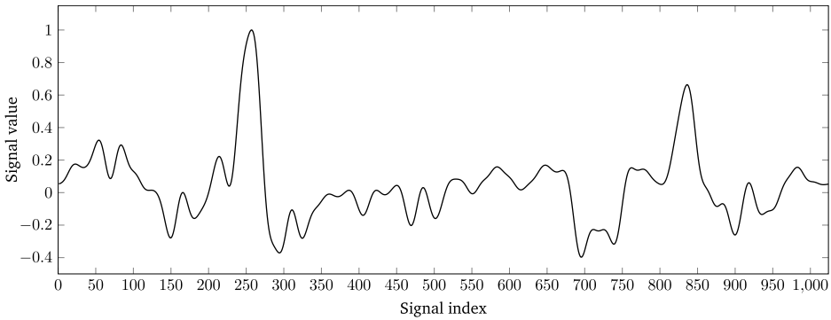
Fig. 1. Original signal \bar{x} .
