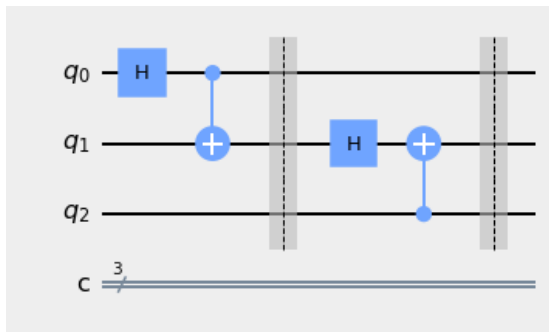
Fig 6. Entangled qubits ready for transmission
