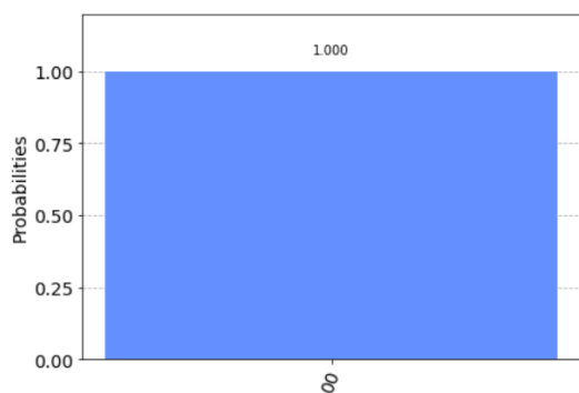
Fig 3. Probability of 1.0 after two Hadamard
