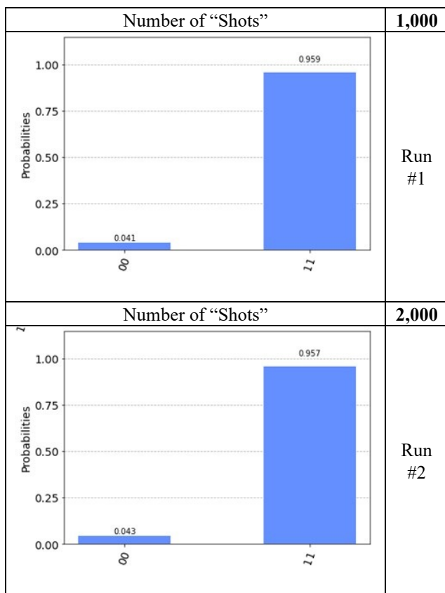
Fig 7. Probabilities 00 and 11 after 1,000 and 2,000 “shots” following a Bell State reversal
