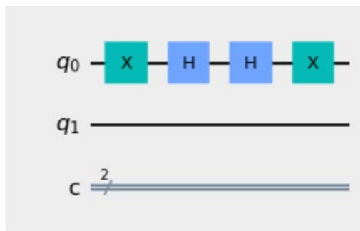
Fig 2. Pauli-X and Hadamard gates applied to q_0
