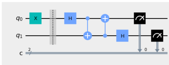
Fig 6. Encoded Quantum Bell State reversed
