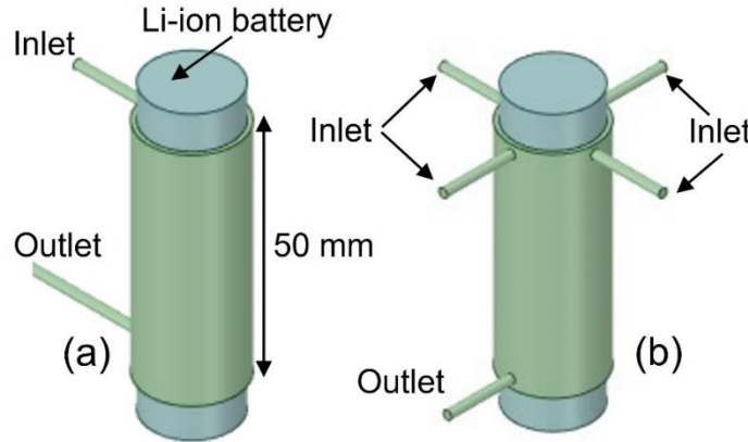
Fig. 1: Three-dimensional view of: (a) one-inlet TMS; (b) four-inlet TMS.
