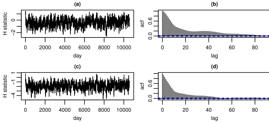
Fig. 8. A time series plot of \mathcal{H} = \mathcal{S}_{50}^{\text{avg}} \circ \mathcal{D}_{10}^{\text{min}} is shown in (a), while (b) shows the corresponding ACF plot, for the site in Wyoming. Panels (c) and (d) show the same information for \mathcal{H} = \mathcal{S}_{50}^{\text{min}} \circ \mathcal{D}_{10}^{\text{min}} .
