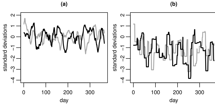
Fig. 5. Time series produced by applying duration functionals \mathcal{D}_\ell to the standardized temperatures for the Wyoming site using \ell = 10 . Time series having the same color correspond to the same year. Panel (a) shows the 10-day running means \mathcal{D}_{10}^{\text{avg}}(Z_n)(\mathbf{s}_i, t_k) as a function of k = 1, \dots, 365 for two different years. Panel (b) shows the 10-day running minimum, based on the \mathcal{D}_{10}^{\text{min}} functional applied to the same data.
