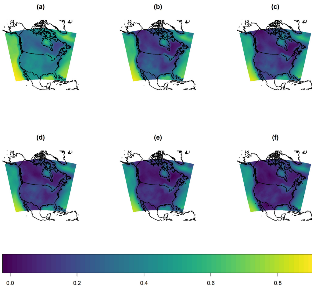
Fig. 14. A heat map of the autocorrelation function of \mathcal{H} = S_d^{\min} \circ \mathcal{D}_\ell^{\text{avg}} for several lags, with \ell = 10 days and smoothing over d = 50 nearest neighbors. The autocorrelation function is shown for lags of (a) 10, (b) 20, (c) 30, (d) 40, (e) 50, and (f) 60 days.
