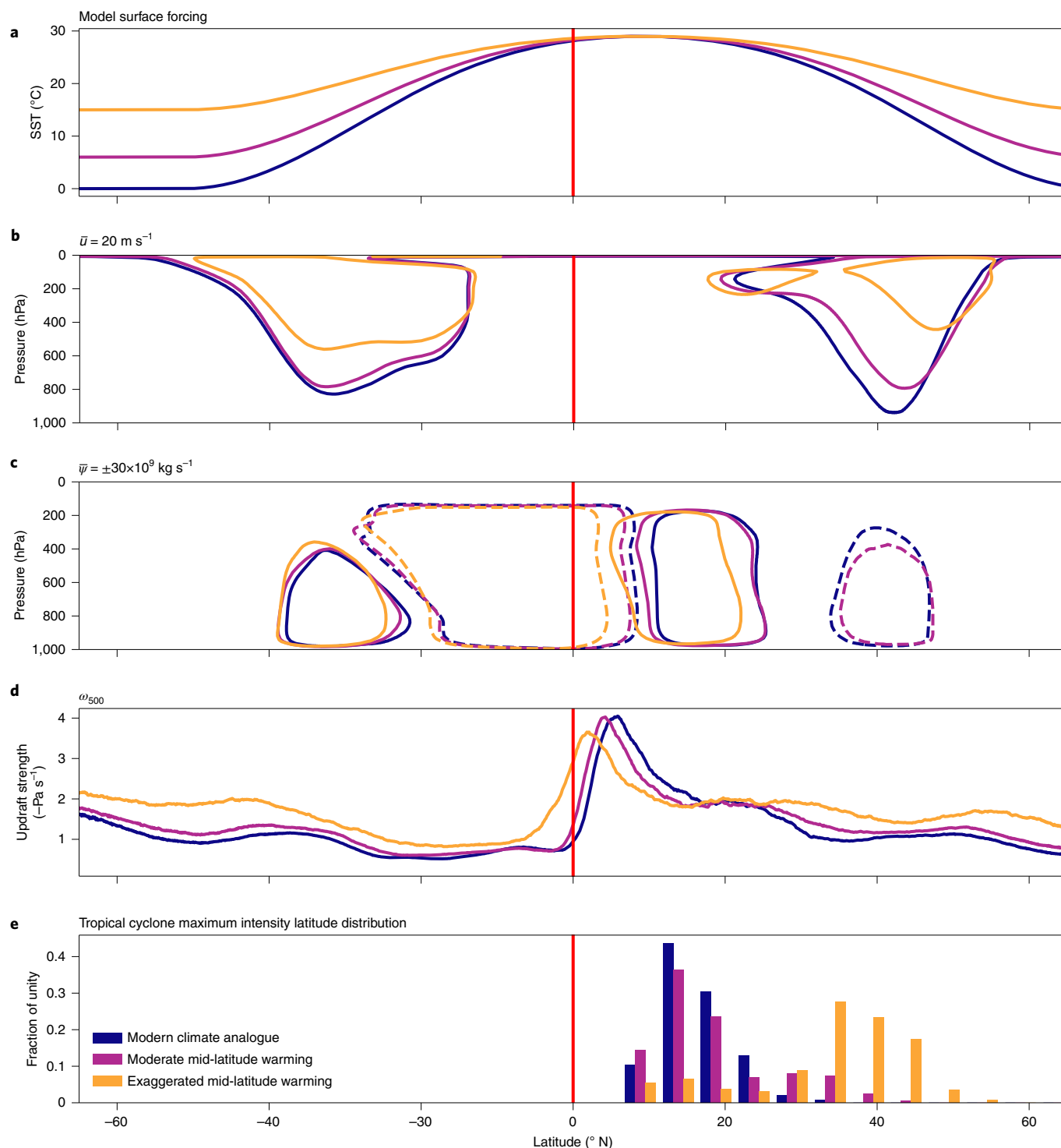
Fig. 5 | Large-scale circulations and TC latitudinal distributions under idealized climate warming scenarios in cloud-system-resolved aquaplanet simulations. a , The model is forced by three fixed SST meridional profiles that range from contemporary climate (blue) to moderate mid-latitude warming (purple) to exaggerated Eocene-like warming (orange). b , \bar{u} = 20 \text{ m s}^{-1} zonal velocity contours that mark the jet streams. c , \bar{\psi} = \pm 30 \times 10^9 \text{ kg s}^{-1} streamlines of the Hadley and Ferrel cells. d , Mean updraft strength measured as the time mean of the zonal maximum pressure velocity at 500 hPa multiplied by -1. e , Divergent influences lead to the northward shift of TC LMI distribution (despite non-monotonic changes at low latitudes). Data from Fedorov et al. 32 , who also found that GPI calculations underestimate the magnitude of the mid-latitude genesis response to warming.
