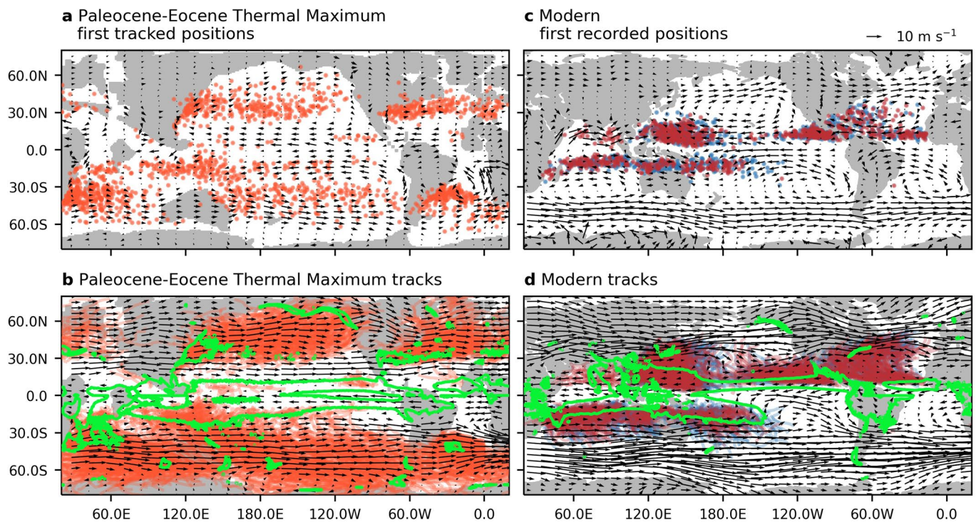
Extended Data Fig. 4 | Planetary-scale atmospheric circulation, precipitation, and TC activity during the simulated Paleocene-Eocene Thermal Maximum (PETM) and the modern period. a, c First tracked positions and b, d TC tracks for PETM and modern climates. The green overlay in b and d show the 6.5 mm/day climatological TC season precipitation contours. PETM data is replotted from simulations in ref. 34 and modern data is from IBTrACs (methods). Red and blue dots are as in Fig. 2, blue for 1980-1999 and red for 2000-2019. Note that the lysis definition marking the end of the tracks between the PETM tracking and modern data are not easily reconcilable. The suppression of the low latitude TCs in the PETM is related to the splitting of the summertime subtropical and eddy-driven jets (Extended Data Fig. 5 and Fig. 5).
