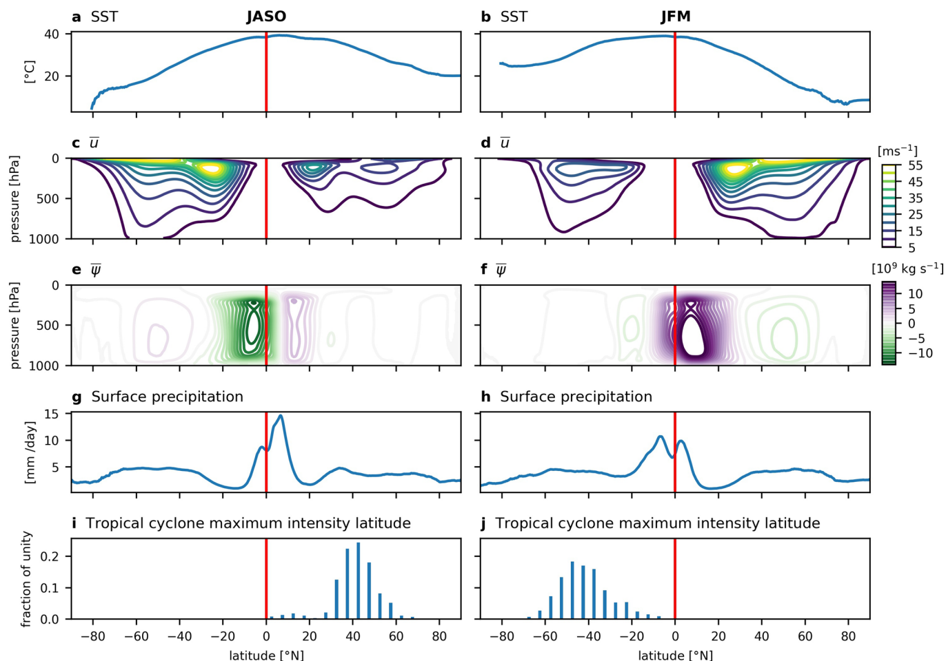
Extended Data Fig. 5 | Zonal-mean large-scale climate and north-south TC lifetime maximum intensity during the Paleocene-Eocene Thermal Maximum (PETM, \text{CO}_2 1590 ppm). Replotted from the \sim 0.25 -degree resolution atmospheric GCM simulations of ref. 34 . Note the strong agreement on coincident jet split and TC activity in the midlatitude with the idealized cloud-system-resolving aquaplanet simulations of ref. 32 shown in Fig. 5 of the main manuscript.
