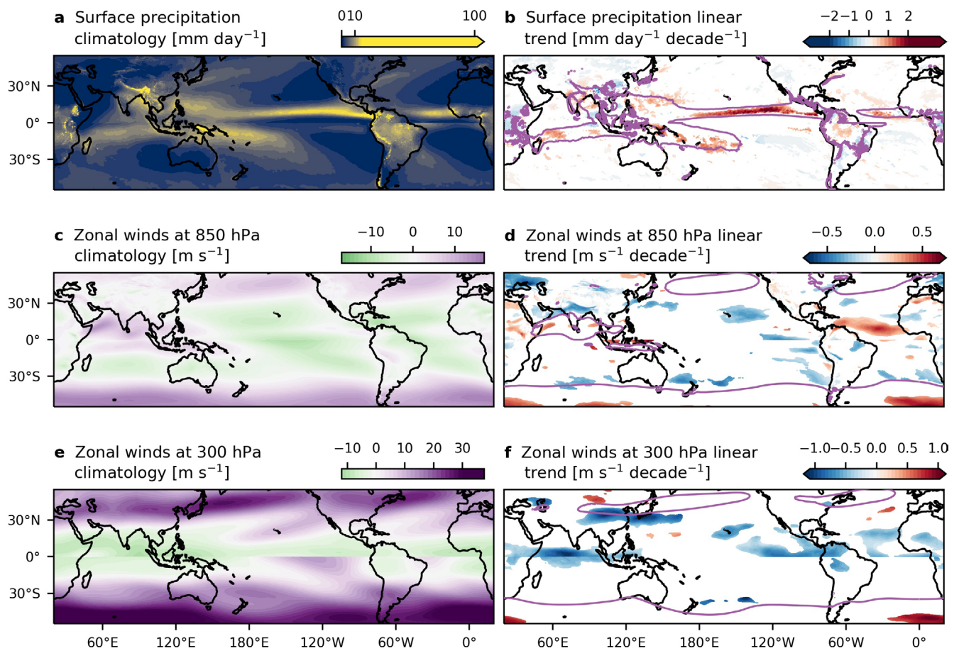
Extended Data Fig. 6 | Surface precipitation, tropospheric winds and recent linear trends from ERA5. a, c, e The 1980–2019 precipitation, and upper (300 hPa) and lower level (850 hPa) wind climatologies for the tropical cyclone season (July through September for the northern hemisphere, January through March for the southern hemisphere). b, d, f The linear trends in these climatologies over the same period. Only trends for which p values are < 0.05 are plotted. The contour lines in b, d , and f are used to visualise the ITCZ ( 6.5 \text{ mm day}^{-1} ), and the jet stream locations ( 5 \text{ m s}^{-1} in the lower troposphere in d and 20 \text{ m s}^{-1} in the upper troposphere in f ). Data from ERA5 156 .
