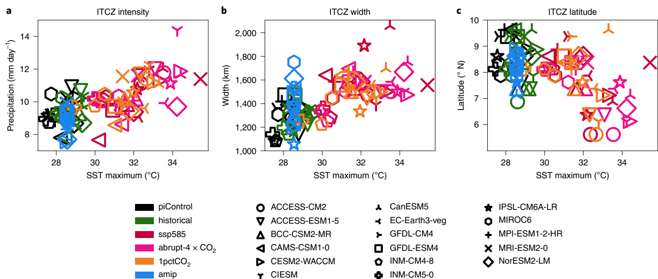
Fig. 6 | Changes in the Northern Hemisphere ITCZ under different warming scenarios in CMIP6. a–c, ITCZ intensity (a), width (b), and latitudinal position (c). For higher tropical SSTs, as predicted for the twenty-first century, climate models predict a stronger and broader ITCZ that is shifted towards the equator (Methods and see Extended Data Fig. 7 for changes in the Southern Hemisphere). Data from refs. 158–174 .
