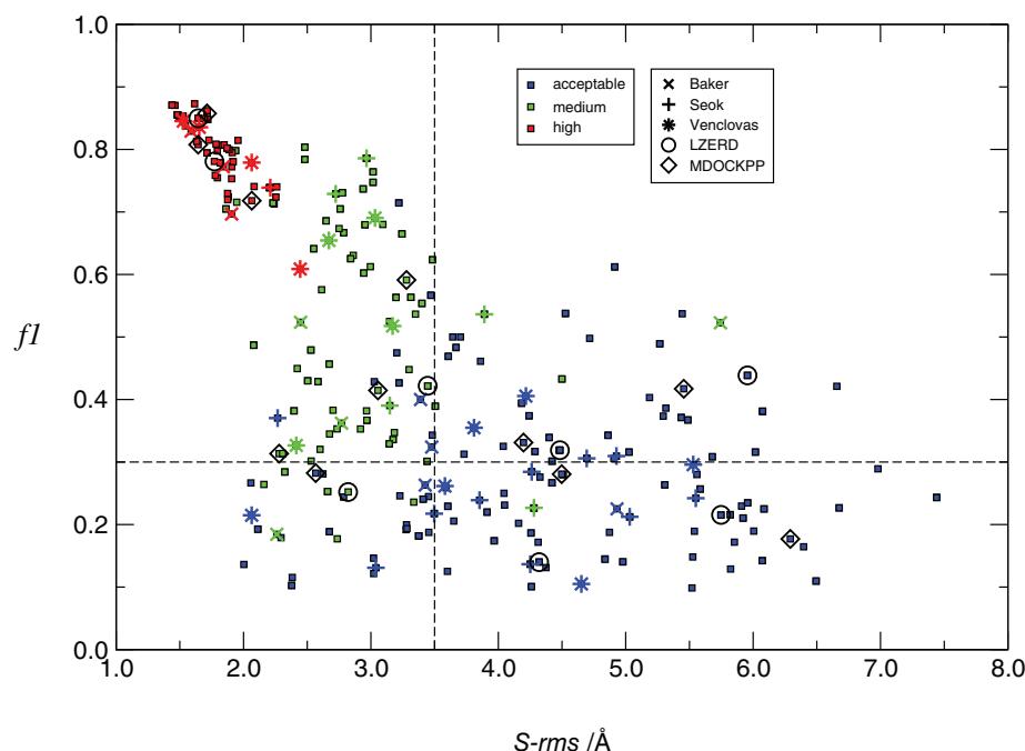
FIGURE 7 f1 as a function of S\text{-rms} . Each point in the figure represents the best model of a predictor group for each of the 23 interfaces. Individual points are color-coded following the CAPRI model quality as in Figure 6. The results for the best predictors (Baker, Seok, and Venclovas) and servers (LZERD, MDOCKPP) are highlighted. See main text for definition of f1 and S\text{-rms} . The upper left quadrant features the best models, with S\text{-rms} values below 3.5 Å and f1 values above 0.3, corresponding to mostly medium and high-quality models
