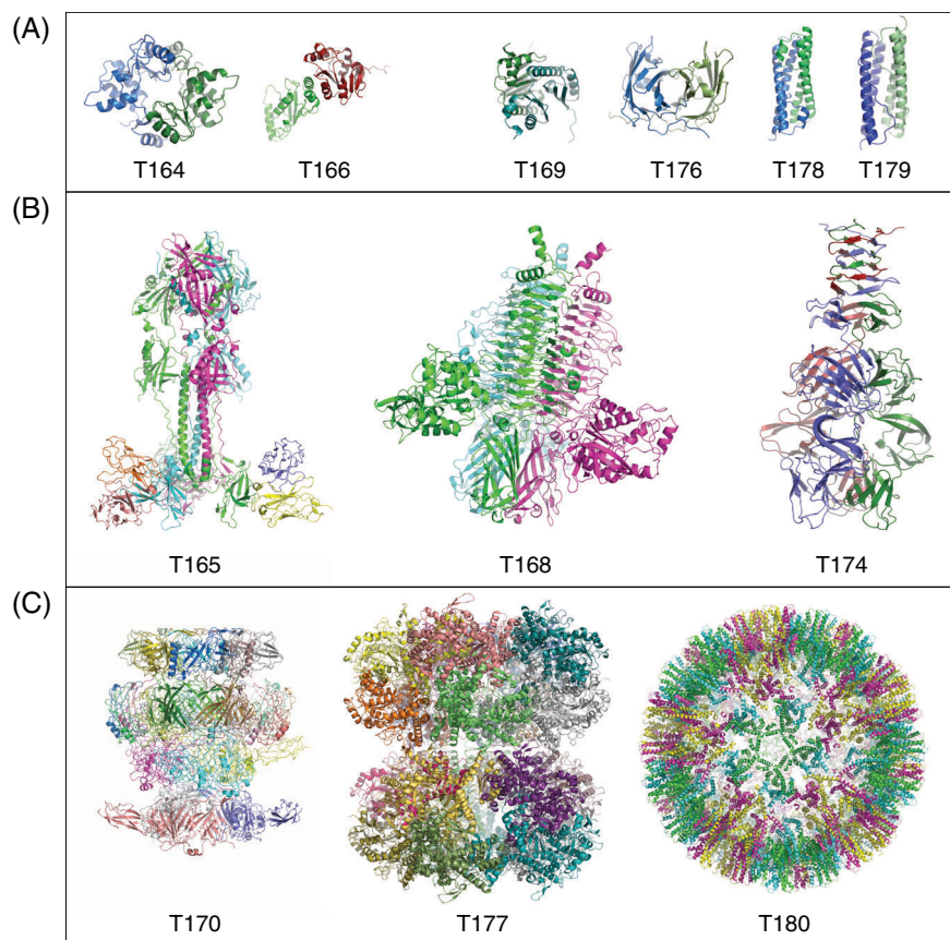
FIGURE 1 The Targets of Round 50. (A) Dimeric targets, (B) trimeric targets, (C) large assemblies. The dimeric targets are divided into Easy (T164/T1032 and T166/H1045) and Difficult (T169/T1054, T176/T1078, T178/T1083, and T179/T1087) targets. The trimeric targets T165/H1036 and T174/T1070 were Difficult, whereas T168/T1052 was easy. The large assembly target T177/T1081 was an easy target. The remaining targets T170/H1060 and T180/T0199 featured both Easy and Difficult to predict interfaces
