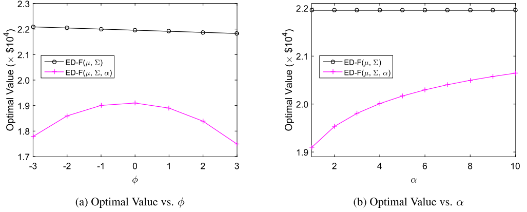
Fig. 2. Optimal values of ED-F(\mu, \Sigma) and ED-F(\mu, \Sigma, \alpha) with various \phi and \alpha (adapted from Figure 3 of [130]).
