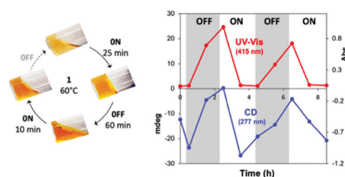
Fig. 4 Temporal evolution of the assembly/disassembly cycle of 1 (3 mM) at 60 °C (90 mM TFA). Formation and breakdown of the hydrogel (left) and CD and UV-Vis signals (right) at 277 and 415 nm, respectively, with each on/off cycle of visible light illumination.
