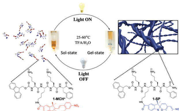
Fig. 1 Transient self-assembly of nanofibers driven by visible light as fuel. Scheme of the reaction network showing interconversion between the metastable spiropyran (SP) form and the merocyanine (MCH) resting state of 1 .
