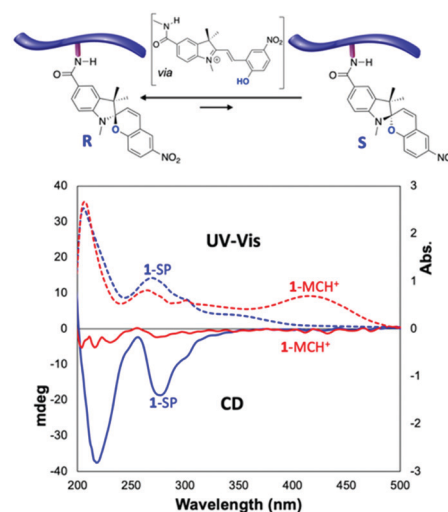
Fig. 3 Rapid interconversion of R and S -spiropyran centers of 1-SP via the intermediacy of the planar MCH + form. UV-Vis and CD spectra of 1-SP hydrogel and 1-MCH + . Samples of 1-SP or 1-MCH + were formed in water (3 mM, 90 mM TFA) at 60 °C, either under continuous illumination with visible light for 1-SP , or in the dark for 1-MCH + , then diluted to 0.6 mM prior to recording the spectra.
