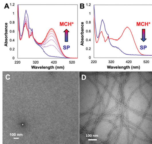
Fig. 2 Interconversion of merocyanine and spiropyran forms of 1 in water (0.3 mM, 90 mM TFA), as monitored by the increase/decrease of the MCH + UV-Vis absorption at 415 nm. (A) 1 -SP heated at 60 °C in the dark and absorption recorded at 10 min intervals over 70 min. (B) Irradiation of 1 -MCH + with visible light for 1 min at room temperature (LED, 60 W). TEM images of 1 in water (3 mM, 90 mM TFA) (C) after heating to 60 °C for 60 min in the dark, (D) and after irradiation with visible light for 24 h in water (3 mM, 90 mM TFA) at 60 °C.
