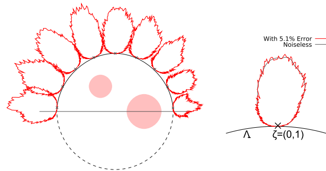
Figure 6. Boundary data u|_{\Lambda_+} with relative 5.1% errors in L^2 sense; (left) the measurement arc \Lambda lies in the upper half plane; (right) comparison of u(\zeta, \theta) at \zeta = (0, 1) between 5.1% noisy data (red) and the original data (gray) in figure 2.
