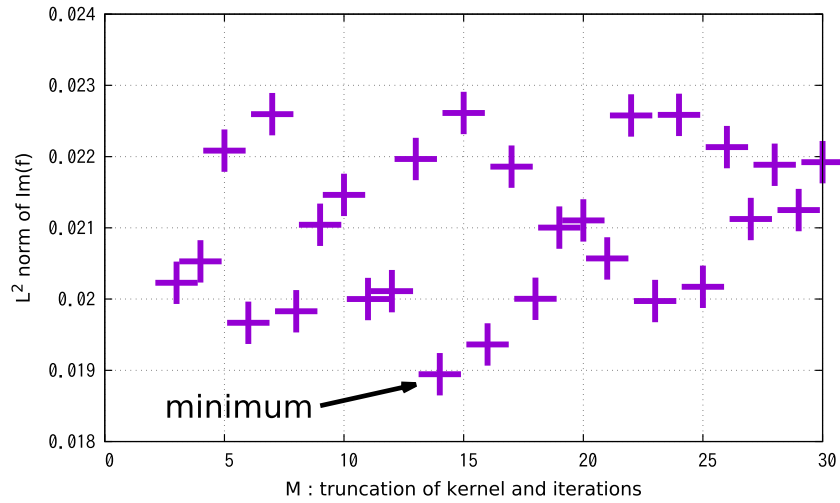
Figure 7. L^2 norm of the imaginary part of the reconstructed f from measurement data with added 5.1% relative error, and a varying cutoff parameter 0 \leq M \leq 30 . At M = 14 the minimum is achieved.
