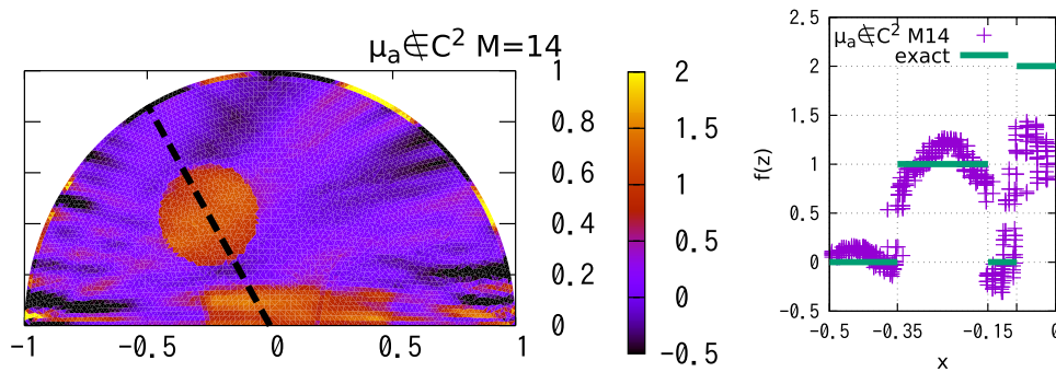
Figure 8. Numerically reconstructed f(z) for measurement data 5.1% errors in figure 6 with discontinuous \mu_a (47) and Poisson kernel (48).
