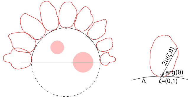
Figure 2. Boundary data u|_{\Lambda_+} : (left) the measurement arc \Lambda lies in the upper half plane. Each red closed curve stands for \zeta + 2u(\zeta, \theta) for \theta \in \mathbf{S}^1 at \zeta \in \Lambda indicated by the cross symbol ( \times ); (right) magnification of u(\zeta, \theta) at \zeta = (0, 1) .
