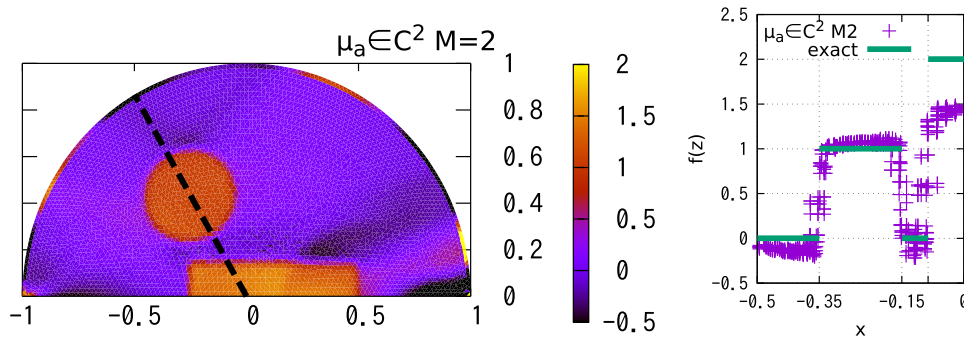
Figure 3. Numerically reconstructed f(z) for polynomial type scattering kernel (46) and \mu_a \in C^2(\Omega) . (left) The profile of reconstructed f in the domain of interest \Omega^+ ; (right) the section on the dotted line.
