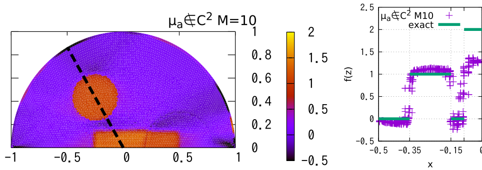
Figure 5. Numerically reconstructed f(z) for the case with discontinuous \mu_a (47) and Poisson kernel (48).
