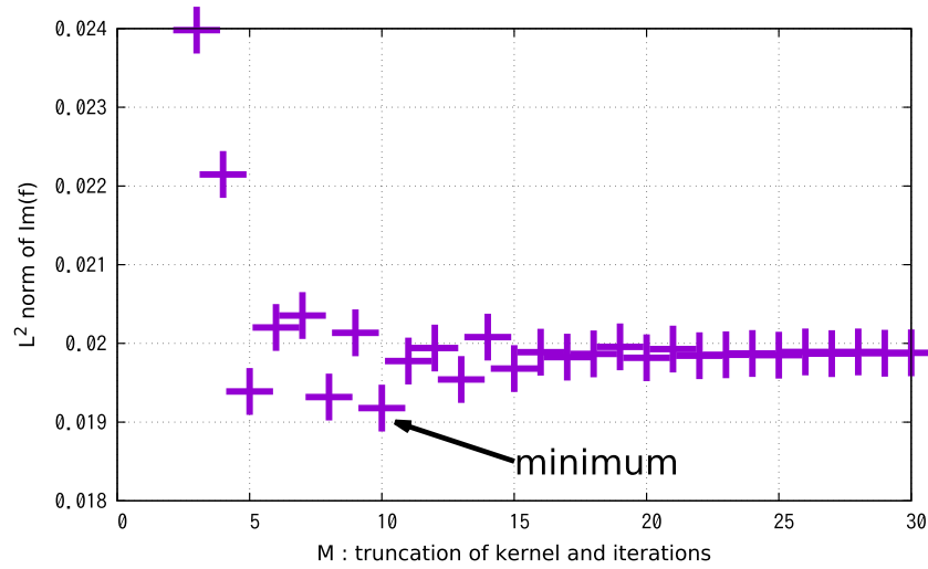
Figure 4. L^2 norm of the imaginary part of the reconstructed f for varying cutoff parameter M in the range 0 \leq M \leq 30 . The minimum is attained at M = 10 . The values for M = 0, 1, 2 are greater than 0.024, and are not shown in the graph.
