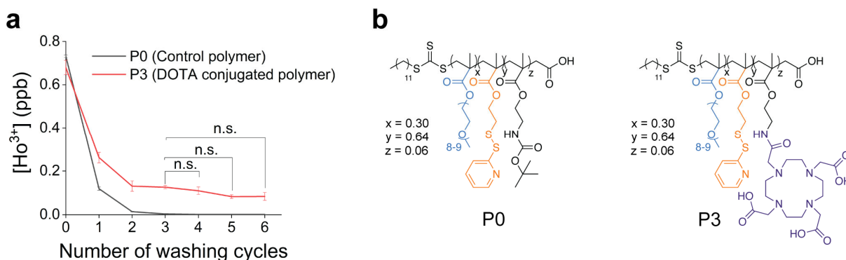
Figure 2. (a) ICP-MS analysis after \text{Ho}^{3+} complexation of P3 and the control polymer P0 for a different number of washing cycles. Three washing steps were enough to remove free, non-specifically bound \text{Ho}^{3+} , as indicated by the undetectable levels of \text{Ho}^{3+} in P0. The abbreviation n.s. indicates no significant difference in the signals. (b) Chemical structures of control polymer (i.e. P0) and DOTA conjugated polymer (i.e. P3).
