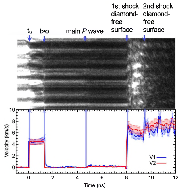
Figure 5. Velocimetry data from reverberation compression of water to ~200 GPa. Example raw VISAR1 (blue line & streak camera image) and VISAR2 (red line) data from Run 209 over a 28 \mu\text{m} region showing particle velocity ( U_p ) of the diamond ablator ( \sim 4.5 \text{ km s}^{-1} ) and free surface velocities ( U_{fs} ) from the 1st and 2nd shock arrivals at the diamond VISAR window ( \sim 7\text{--}7.5 \text{ km s}^{-1} ) ranging from 4.4 to 6 \text{km s}^{-1} . Due to VISAR quality, the U_p uncertainty is \sim 10\% . Breakout (b/o) of the diamond elastic wave into the water layer occurs at \sim 1.5 \text{ ns} , followed by the main pressure wave reaching the VISAR-side diamond-water interface at \sim 4.5 \text{ ns} . The 1st and 2nd shockwave arrivals reach the VISAR-side diamond-vacuum interface at \sim 8 \text{ ns} and 9.5 \text{ ns} , respectively. Drive laser parameters listed in Table 2.
