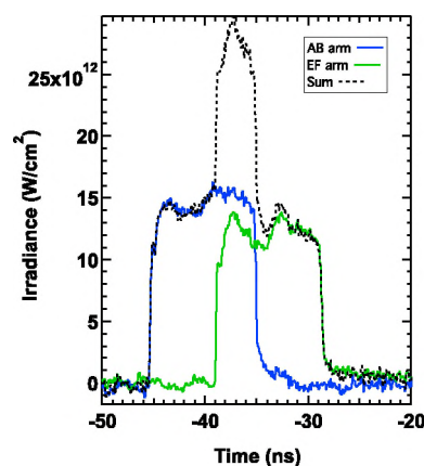
Figure 6. Oscilloscope traces of drive laser temporal profiles. Blue and green traces show the two 10 ns flat-top profiles offset by \sim 5 \text{ ns} to yield a stepped \sim 15 \text{ ns} drive pulse profile. Two separate laser ‘arms’ are combined to generate the compression wave, here labeled AB and EF corresponding to names of the capacitor banks. The total irradiance as seen by the target is the sum of the two drive profiles shown by the dotted black line.
