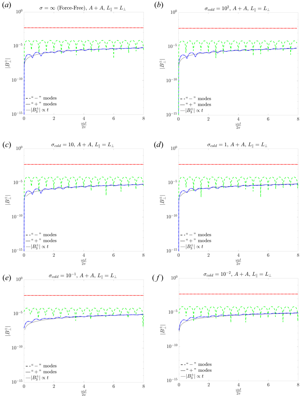
FIGURE 1. Mode evolution of B_{\perp} for a cubic domain with \chi = 0.01 and \sigma_{cold} \equiv b^2/\rho \in [0.01; 0.1; 1; 10; 100; \infty] , presented in descending order of \sigma from (a) to (f). The red lines correspond to the initial counter-propagating Alfvén modes: the (0, 1, -1) and (1, 0, 1) modes are shown by dashed and dotted lines, respectively. Dashed green lines correspond to the second-order nonlinear shear mode (1, 1, 0) . The (1, 2, -1) and (2, 1, 1) third-order, secularly growing modes are shown by dashed and dotted blue lines, respectively. The black line corresponds to a secular growth directly proportional to t and scaled by the final amplitude of the third-order mode.
