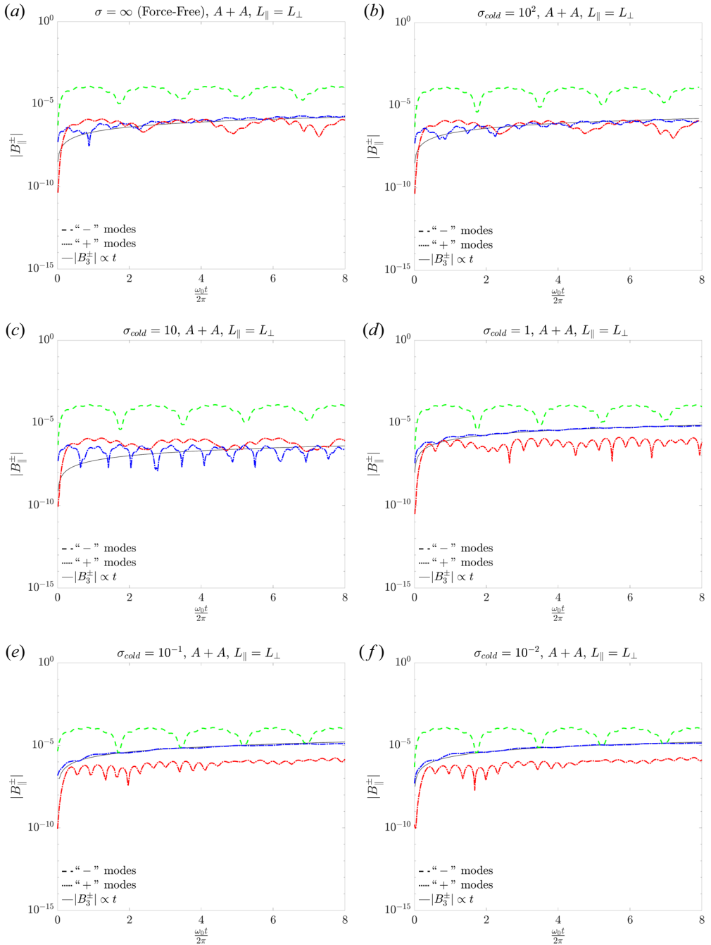
FIGURE 2. Mode evolution of B_{\parallel} for a cubic domain with \chi = 0.01 and \sigma_{cold} \equiv b^2/\rho \in [0.01; 0.1; 1; 10; 100; \infty] , presented in descending order of \sigma from (a) to (f). Line styles and colours are as defined in figure 1.
