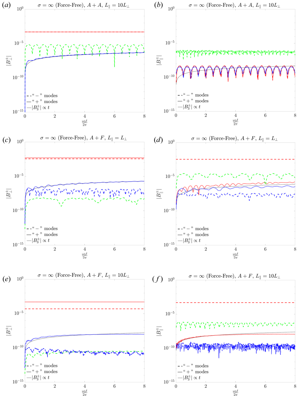
FIGURE 3. Mode evolution of B_{\perp} and B_{\parallel} with \chi = 0.01 . (a,b) Results for an Alfvén wave–Alfvén wave collision in an elongated domain, L_z = 10L_x . (c–f) Results for an Alfvén wave–fast wave collision in a cubic domain (c,d) and elongated domain (e,f). The line style and colour are as in previous figures.
