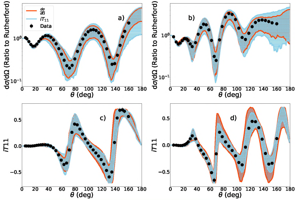
FIG. 6: 95% confidence intervals calculated using \frac{d\sigma}{d\Omega} data (red bands) or iT_{11} data (blue bands) in the optimization procedure: a) d\sigma/d\Omega for ^{48}\text{Ca}(p,p) at 12 MeV; b) d\sigma/d\Omega for ^{48}\text{Ca}(p,p) at 21 MeV; c) iT_{11} for ^{48}\text{Ca}(p,p) at 12 MeV; d) iT_{11} for ^{48}\text{Ca}(p,p) at 21 MeV.
