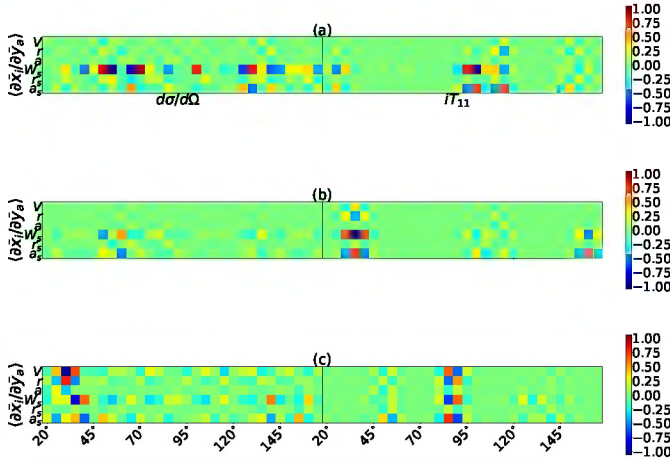
FIG. 7: Sensitivity matrix for \frac{d\sigma}{d\Omega} data and iT_{11} data: a) ^{48}\text{Ca}(n,n) at 12 MeV; b) ^{48}\text{Ca}(p,p) at 12 MeV and c) ^{48}\text{Ca}(p,p) at 21 MeV. More details can be found in the text.
