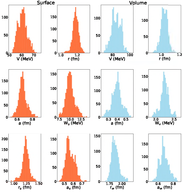
FIG. 1: ^{48}\text{Ca}(p,p) at 9 MeV parameter posterior distributions: surface model (orange) and volume model (blue).
