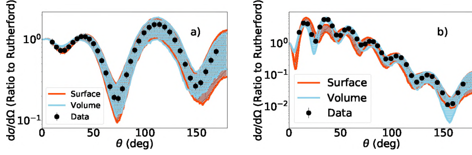
FIG. 3: Angular distribution 95% confidence intervals for \frac{d\sigma}{d\Omega} for ^{48}\text{Ca}(p,p) at (a) 9 MeV and (b) 65 MeV: surface model (orange) and volume model (blue). Mock data generated with [8] (black circles).
