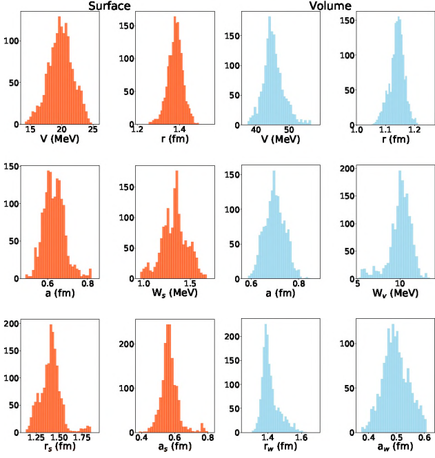
FIG. 2: ^{48}\text{Ca}(p,p) at 65 MeV parameter posterior distributions: surface model (orange) and volume model (blue).
