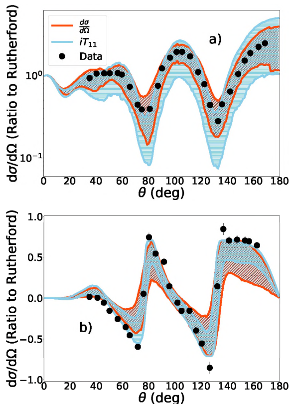
FIG. 8: ^{48}\text{Ca}(p,p) at 14 MeV 95% confidence intervals calculated using \frac{d\sigma}{d\Omega} data (orange bands) or iT_{11} data (blue bands) in the optimization procedure: a) d\sigma/d\Omega and b) iT_{11} . Data from [23].
