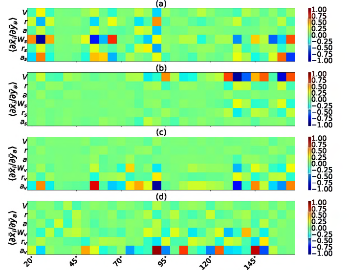
FIG. 5: Parameter sensitivities for ^{48}\text{Ca}(p,p) : a) surface model at 9 MeV, b) surface model at 65 MeV, c) volume model at 9 MeV and d) volume model at 65 MeV.
