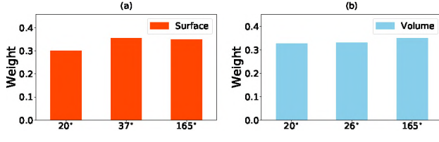
FIG. 4: Principal component analysis for ^{48}\text{Ca}(p,p) at 65 MeV using \frac{d\sigma}{d\Omega} data. Shown are the weights w_a obtained for three different scattering angles: a) for the surface model and b) for the volume model.
