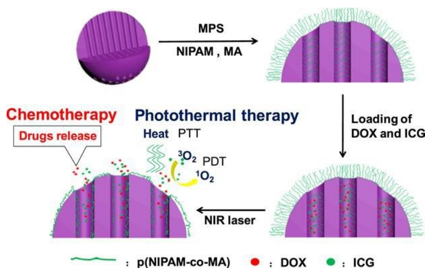
Figure 4. Loading and release of DOX and ICG from MSNs coated with PNIPAM copolymerized with methacrylic acid. The copolymer is abbreviated as p(NIPAM-co-MA). Copolymers are grafted from the surface of the MSN, generating dense brushes across the surface and into the porous interior. While the polymers are hydrated, off-target release is restricted. Upon heating by an externally applied NIR laser, the polymers collapse and release the loaded drug. Reprinted with permission from [143], Elsevier, 2018.
