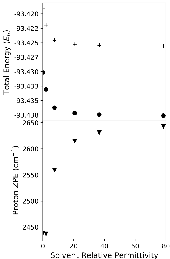
Figure 1. Energetics of HCN in a variety of solvents with a classical proton description (circles) and with a NEO protonic wavefunction (crosses). The protonic zero-point energy is shown with triangles.
