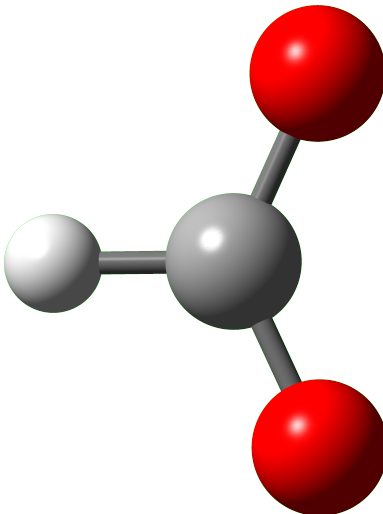
Figure 3. Structure of the formate ion, \text{CO}_2\text{H}^-
