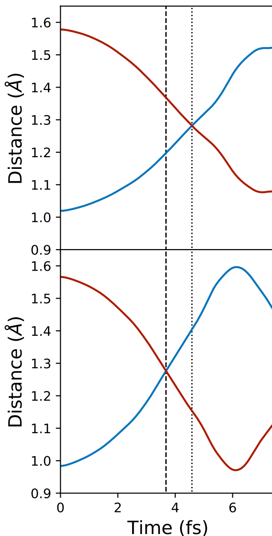
Figure 5. Excited state intramolecular proton transfer in oHBA in vacuum (top) and water (bottom) for the restricted excited state geometry. The distance between the expectation value of the transferring proton position and the donor oxygen (blue) and acceptor oxygen (red) is given as a function of time. The crossing time in vacuum is marked with the vertical dotted line, and the crossing time in water is marked with the vertical dashed line.
