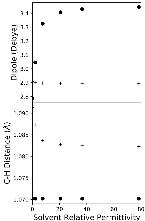
Figure 2. Total molecular dipole moment (top) and C-H bond length (bottom) of HCN in a variety of solvents with a classical description (circles) and with a NEO protonic wavefunction (crosses).
