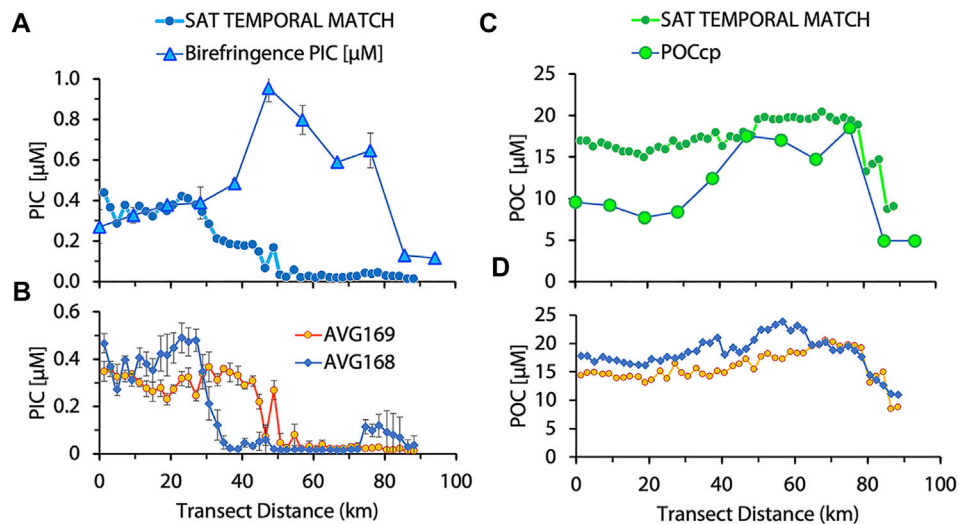
FIGURE 13 | (A) Comparison of surface layer PIC concentrations derived from PIC011 along Transect T2 with time interpolation of PIC retrieved from VIIRS SNPP satellite data from days 168 and 169. (B) PIC retrieved from VIIRS SNPP satellite data from days 168 and 169. (C,D) similar comparisons for POC derived from transmissometer beam attenuation coefficient and satellite retrievals. In the case of PIC, the satellite retrieval of PIC agreed well along the first 30 km of the transect and then strongly diverged to near zero values while sensor PIC reached concentrations of 1 μM. Retrievals of POC from CTD casts and satellite data were far more in agreement.
