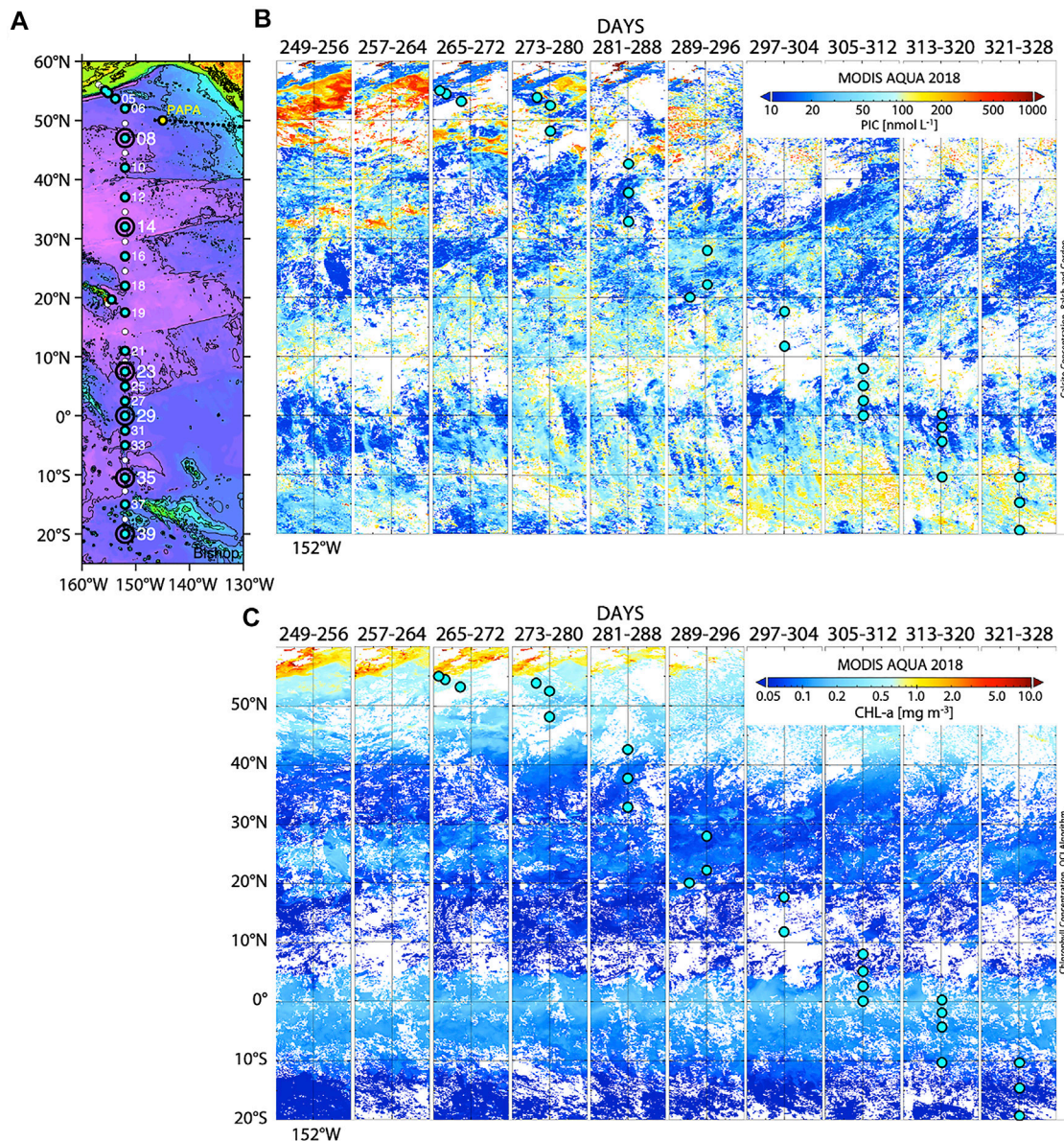
FIGURE 2 | Spatial and remote sensing context for the September to November 2018 GEOTRACES GP15 transect from Adak Alaska to Tahiti. Stations where the McLane large volume in situ filtration system was deployed are denoted by cyan-filled symbols. Stations ringed with a large circle denote locations with three casts ( A ). The GEOTRACES Trace Element Carousel (GTC CTD) was deployed at all stations. ( B ) shows MODIS AQUA satellite retrievals of PIC averaged over 8 days from 60°N to 20°S and from 147°W to 157°W at 4 km resolution over the time of the transect. The UTC day range for each swath is shown at the top of each swath. Station locations are mapped onto the contemporaneous swath. ( C ) shows similar swaths for MODIS AQUA chlorophyll. Plots were made using Panoply, an application of the NASA Goddard Institute for Space Studies.
