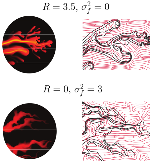
FIG. 3. Difference in the finger tip structures between fingering-dominated ( top row ) and heterogeneity-dominated ( bottom row ) flows. The left column shows the concentration fields in the two cases within a zoom-in view window. The right column shows the concentration contours ( black lines ) superposed on the streamlines ( red lines ). Fingering-dominated flows produce rounder and better delineated tips than heterogeneity-dominated flows. Fingering also produces tip splitting that is absent at R = 0 .
