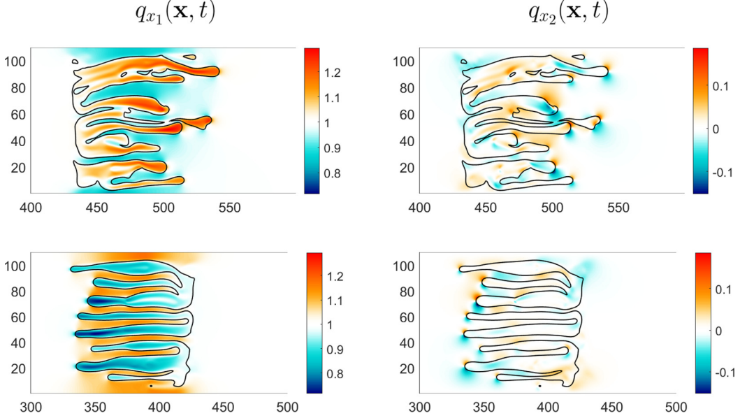
FIG. 5. Longitudinal and transversal velocity fields [q_{x_1}(\mathbf{x}, t) and q_{x_2}(\mathbf{x}, t) respectively] for a solute cloud with viscosity contrast R = 1 (top row) and R = -1 (bottom row) in a homogeneous field. The black lines represent the contour of the solute cloud at a threshold concentration value C = 0.1 .
