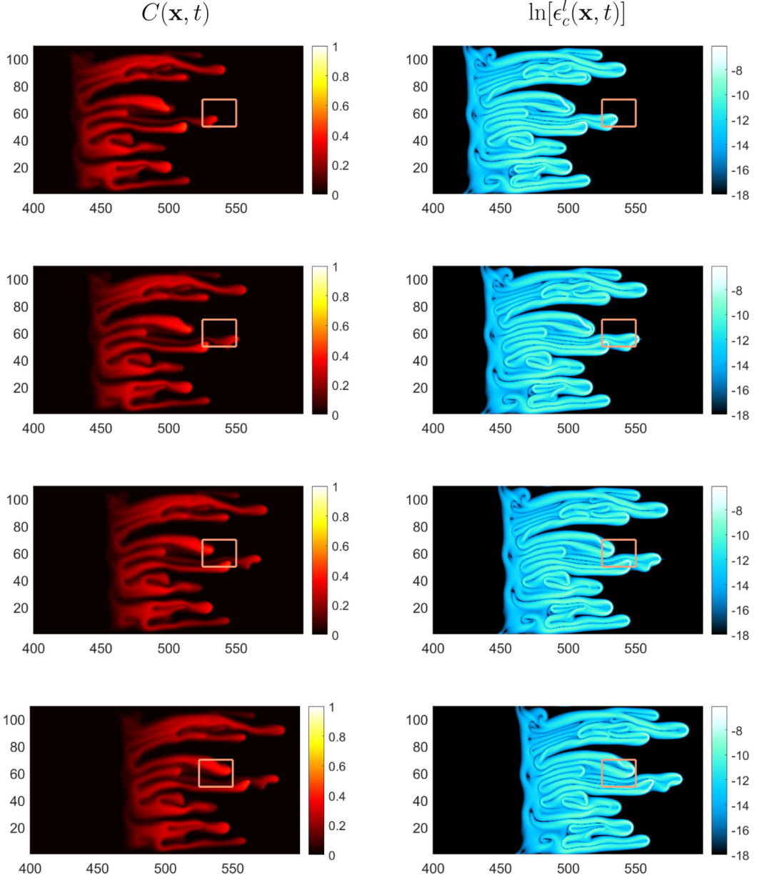
FIG. 2. Concentration field C(\mathbf{x}, t) (left column) and logarithm of the local scalar dissipation rate \epsilon_c^l = \frac{|VC(\mathbf{x}, t)|^2}{\text{Pe}} (right column) at four subsequent time steps (from top to bottom) for a viscosity contrast R = 1 in a homogeneous permeability field. Note how the concentration gradient progresses in the orange square, moving from the bottom left quadrant to occupy the whole bottom half in the first two time snapshots. As another finger enters the region defined by the orange square, the concentration gradient locally increases also in the upper half of the considered square.
