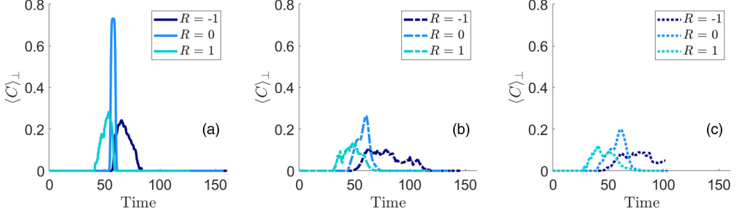
FIG. 7. Breakthrough curves (BTCs) at a control plane located at x_1 = L_{cp} for the three different levels of heterogeneity of the permeability field: (a) homogeneous, (b) heterogeneous with \sigma_f^2 = 0.25 , and (c) heterogeneous with \sigma_f^2 = 0.5 .
