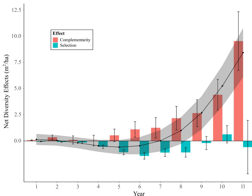
FIGURE 2 Fitted (Equation 3) Net Diversity Effects (NE; Black line ± confidence interval 95% across mixtures and blocks; N = 1100 ) on G ( \text{m}^2/\text{ha} ) over time driven by complementarity and selection effects (red and blue bars respectively ± standard error)
