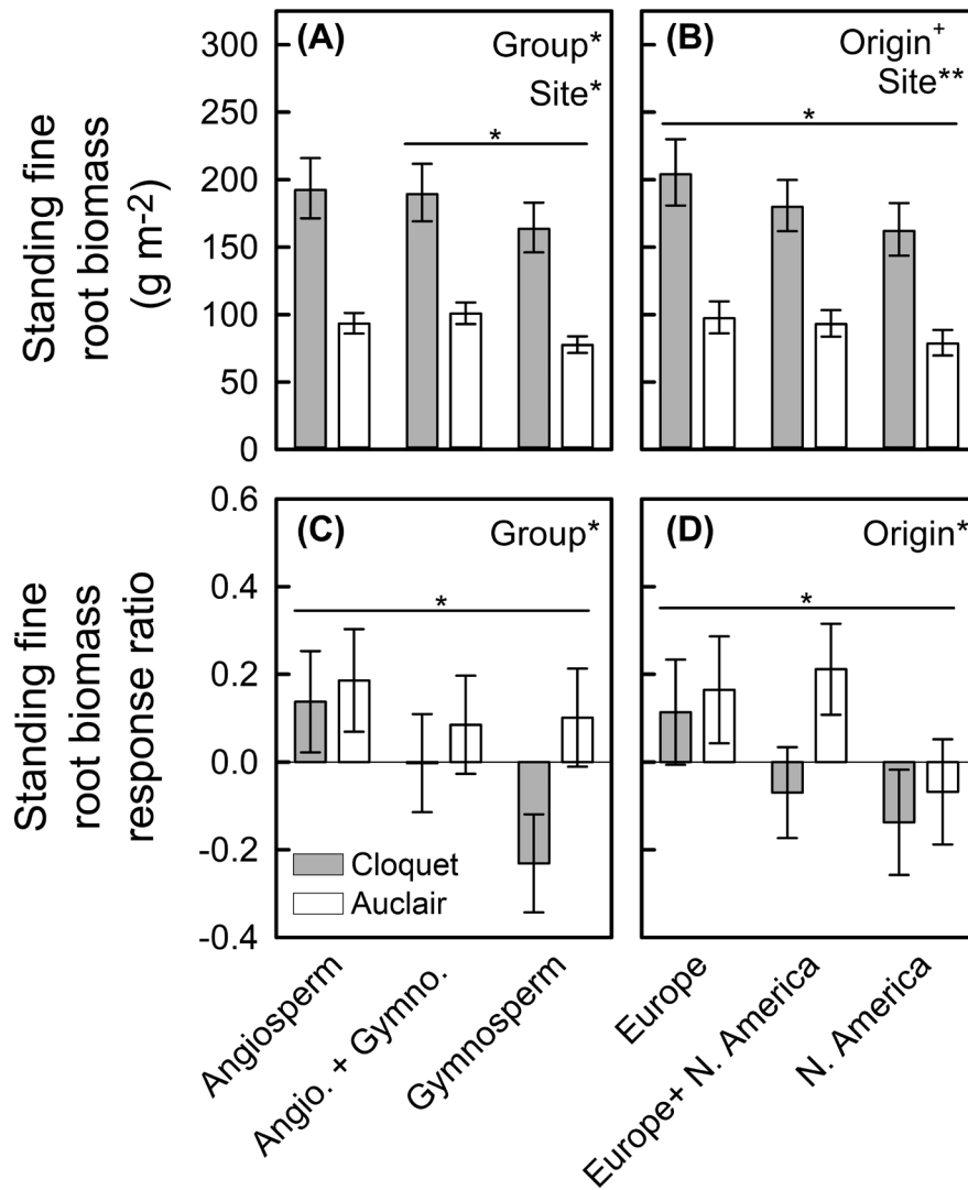
Figure 2. Least-squared mean (± SE) fine-root standing fine-root biomass and standing fine-root biomass response ratios (calculated as (observed – expected)/expected) based on mixture composition: angiosperm only, gymnosperm only or angiosperm–gymnosperm mixtures; or European only, North American only or European–North American mixtures. Includes data from both Cloquet and Auclair sites. Lines indicate statistically distinct values based on group or origin. Effect significance: * indicates 0.05 < p \leq 0.10 , * indicates 0.01 < p \leq 0.05 and ** indicates p \leq 0.01 .
