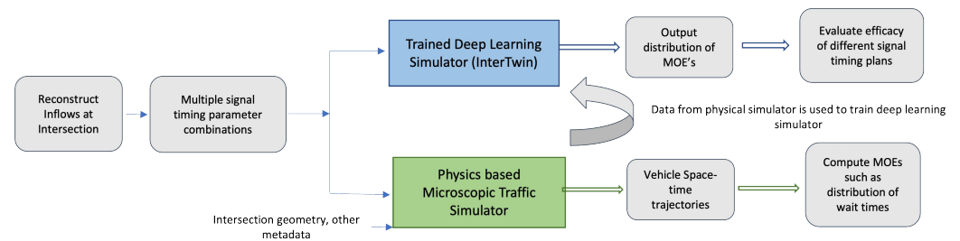
Figure 2. Overall workflow for training the neural network. The data corresponding to different counterfactual signal timing plans is generated using microscopic simulators to train deep neural networks. The trained neural networks can replace the simulators for predicting MOEs such as wait times and are four to five orders of magnitude faster. MOEs: Measures of Effectiveness.
