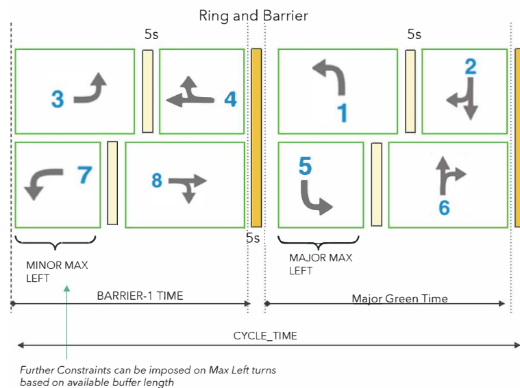
Figure 1. Ring and barrier controller allows us to separate the 8 lane-movements (i.e., phases 1–8) into two concurrency groups, with one group with the major street movements and one for minor street. Key signal timing parameters include cycle time, barrier time, max green splits, etc. For a given input traffic flow, the signal timing parameters are varied to generate different scenarios.
