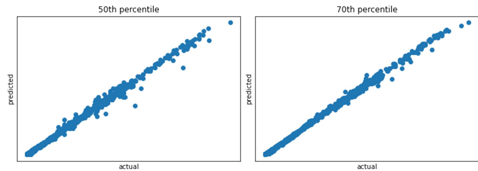
Figure 5. Summary statistics such as 50th/70th percentile etc. can be computed from the predicted distribution. Actual vs. predicted scatter plot of 50th, 70th percentile of wait time computed from the distribution. The key advantage is that predicting distribution enables us to compute any statistic of interest.
