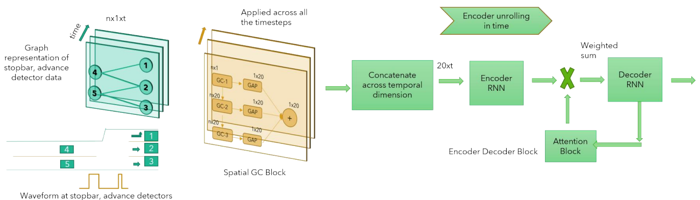
Figure 3. Architecture of the proposed InterTwin model. Spatial Graph Convolution (Spatial GC) is used to extract spatial features from the detector waveforms where the connectivity information of the intersection is incorporated. The encoder-decoder block is used to capture temporal dynamic behavior of the traffic flow.
