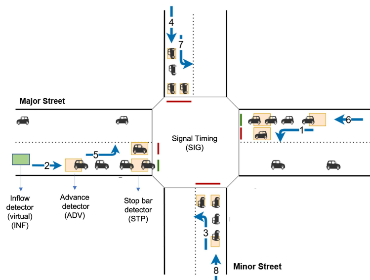
Figure 4. A typical intersection with 8 different directions of vehicular movement (phases 1 to 8). Vehicle waveforms are observed at Stop bar and Advance detectors (STP, ADV). STP, ADV, and INF corresponds to the traffic waveform at stopbar detector, advanced and inflow (500 m away from the intersection) aggregated at a 5-s interval. SIG corresponds to signal timing at a 5-s interval. STP, ADV, and SIG are typically available in ATSPM data for every intersection.
