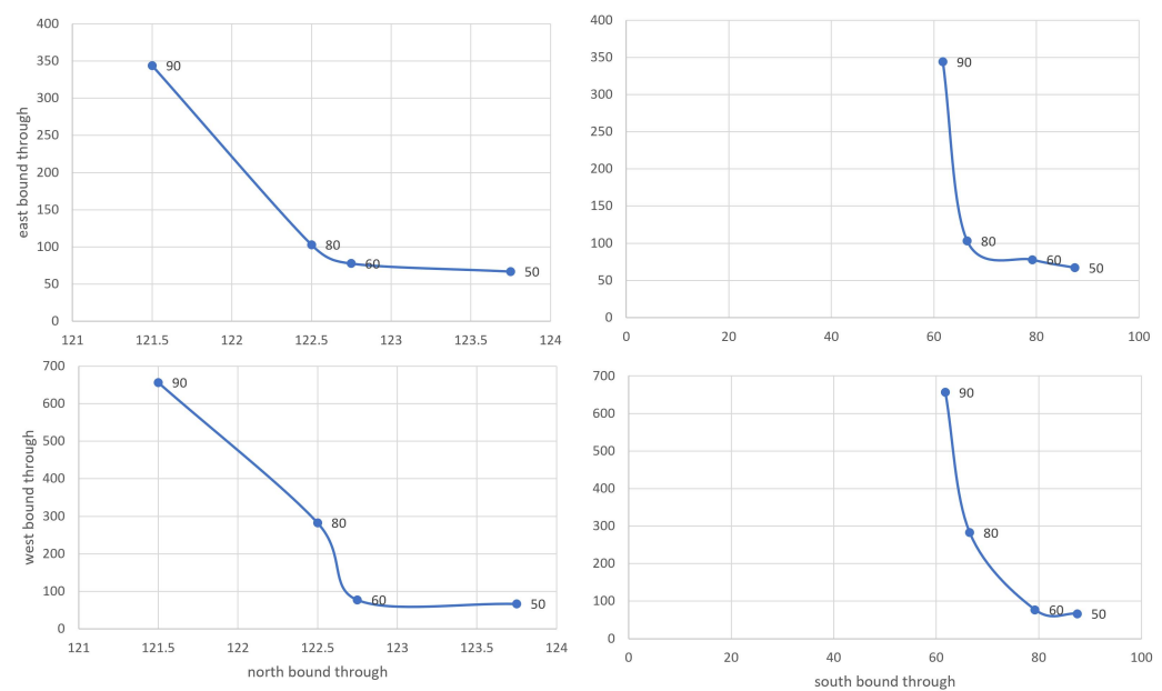
Figure 7. Scatter plot of 75th percentile of wait times for major vs. minor movements for different barrier-1 times. This can be useful to understand trade-offs in wait time for selecting different barrier-1 times for major vs. minor streets.
