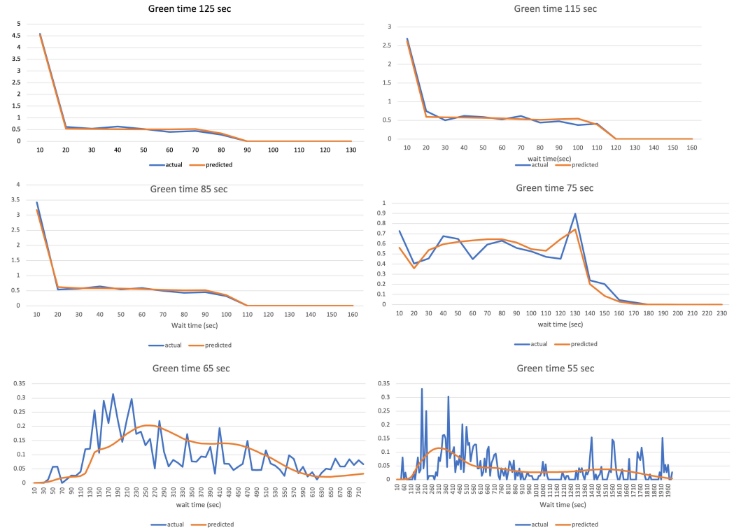
Figure 6. Actual vs. predicted distribution of wait time for different green time splits for a given input traffic. These plots show that the model is able to capture the interrelationship between input traffic and signal timing parameters.
