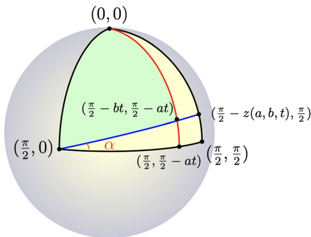
Fig. 2 The deformed triangle T(t) with three vertices at (0, 0) , (\frac{\pi}{2}, 0) , (\frac{\pi}{2} - bt, \frac{\pi}{2} - at)
