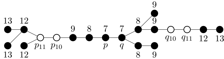
Figure 7. The construction of Theorem 14 applied to a labelled forest F to produce a tree T containing F as a strictly eccentric subgraph. Vertices of F are black and vertices of T - F are white.
