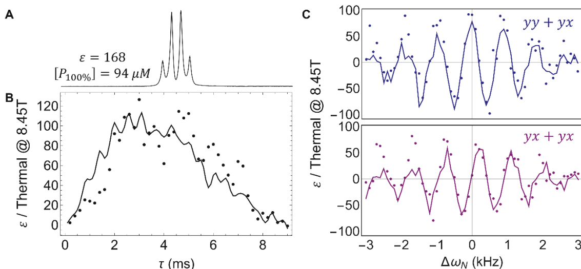
Fig. 5 Experimental performance of broadband phase coherent SABRE sequence using \tau_{HH} = 21 ms. All data were collected using ^{15}\text{N} -acetonitrile (191 mM), pyridine (25 mM), and [\text{Ir}(\text{IMes})(\text{COD})]\text{Cl} (3.7 mM). Simulations (solid lines) assumed a target exchange rate of k_N = 16 s ^{-1} and parahydrogen exchange rate of k_{a,H} = 2 s ^{-1} . A. Hyperpolarized spectrum with a signal enhancement of \varepsilon = 168 using the yy \rightarrow yx excitation phase. This corresponds to a concentration of 100% polarized compound of [P_{100\%}] = 94 \mu\text{M} . B. Scan of the \tau delay of the pulse sequence with the optimum at \tau = 3 ms. The excitation phase used for the pulse sequence was yy \rightarrow yx and \Delta\omega_N \approx (\Delta\omega_{N,b} + \Delta\omega_{N,f})/2 . C. Scan of the ^{15}\text{N} resonance offset pulses using the yy + yx (blue) and yx + yx (purple) steps of the phase cycle.
