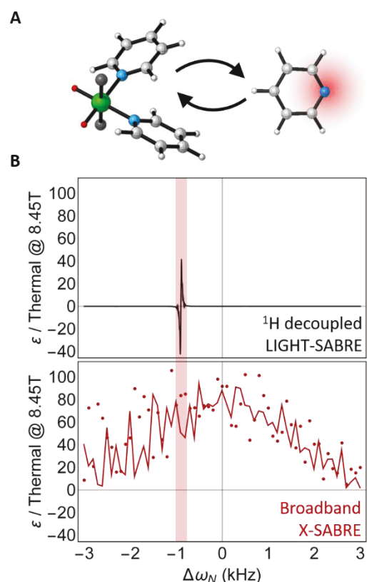
Fig. 1 Top: In SABRE and X-SABRE hyperpolarization methods, a polarization transfer catalyst reversibly binds both para-hydrogen and a molecular target (here shown as pyridine) and singlet order is converted into hyperpolarized target magnetization on the target. Exchanging back into solution forms hyperpolarized free species and polarizes more molecules. Bottom: In previous methods such as ^1\text{H} decoupled LIGHT-SABRE, the hyperpolarization is created by weak irradiation of the iridium-bound heteronucleus, leading to narrow excitation bandwidths. Here, we demonstrate a broadband and phase-coherent excitation strategy that vastly increases hyperpolarization bandwidth. In the broadband case, experimental data are shown with points and simulation is shown by the line.
