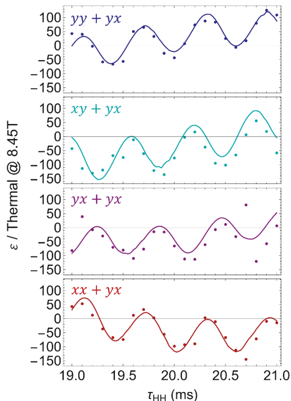
Fig. 6 Hyperpolarization dynamics for the four-steps of the phase cycle required to remove dependence of \hat{\mathcal{H}}_Z when scanning the \tau_{\text{HH}} delay. All data were collected using ^{15}\text{N} -acetonitrile (191 mM), pyridine (25 mM), and [\text{Ir}(\text{IMes})(\text{COD})]\text{Cl} (3.7 mM). Simulations (solid lines) assumed a target exchange rate of k_N = 16 \text{ s}^{-1} and parahydrogen exchange rate of k_{a,H} = 2 \text{ s}^{-1} . Performing the four-step phase cycle allows significantly lower sampling rates when scanning \tau_{\text{HH}} and improving the efficiency of sequence optimization.
