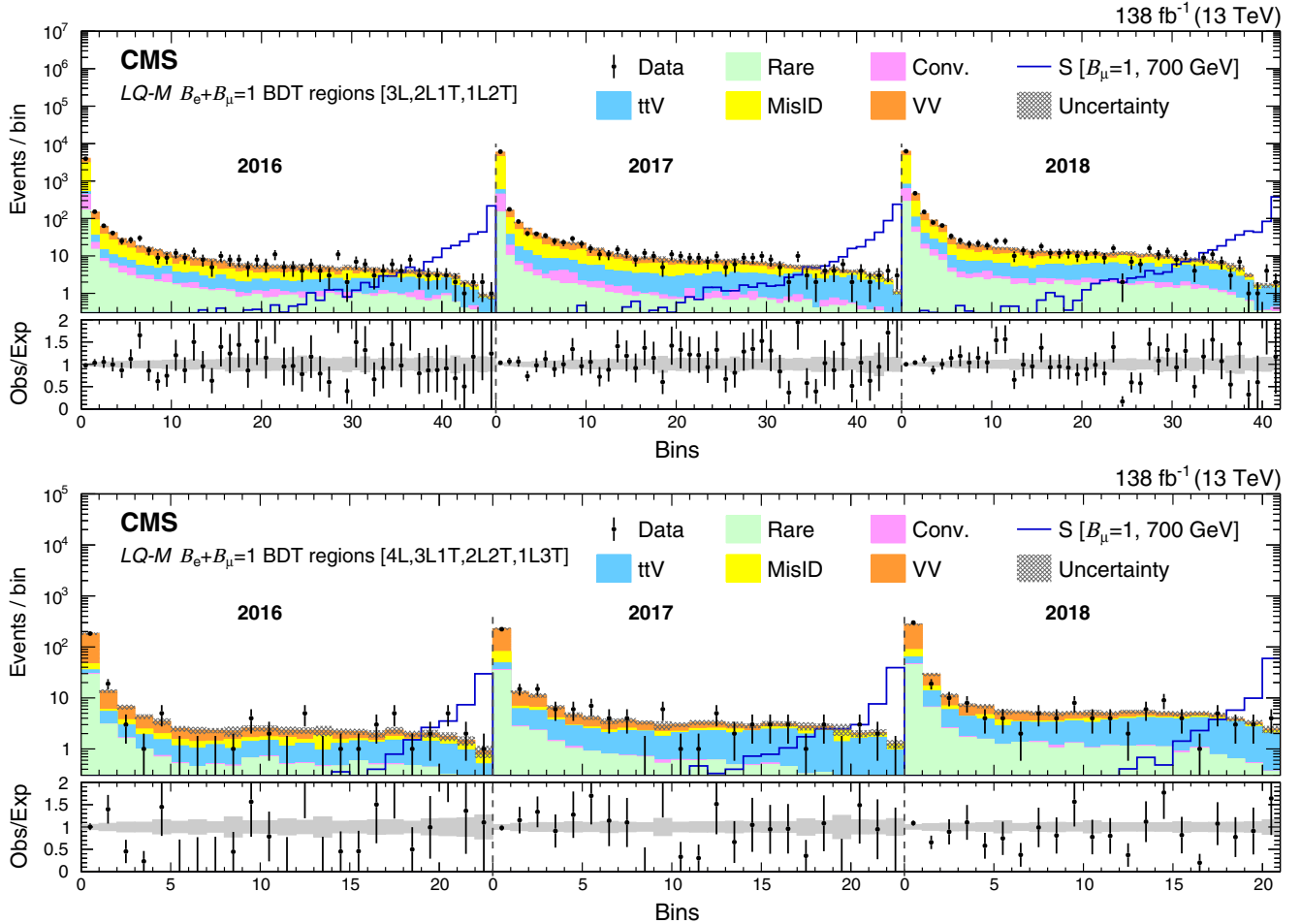
FIG. 22. The LQ\text{-}M B_e + B_\mu = 1 BDT regions for the 3-lepton (upper) and 4-lepton (lower) channels for the 2016–2018 datasets. The lower panel shows the ratio of observed events to the total expected background prediction. The gray band on the ratio represents the sum of statistical and systematic uncertainties in the SM background prediction. The expected SM background distributions and the uncertainties are shown after fitting the data under the background-only hypothesis. For illustration, an example signal hypothesis for the production of the scalar leptoquark coupled to a top quark and a muon for m_S = 700 GeV, before the fit, is also overlaid.
