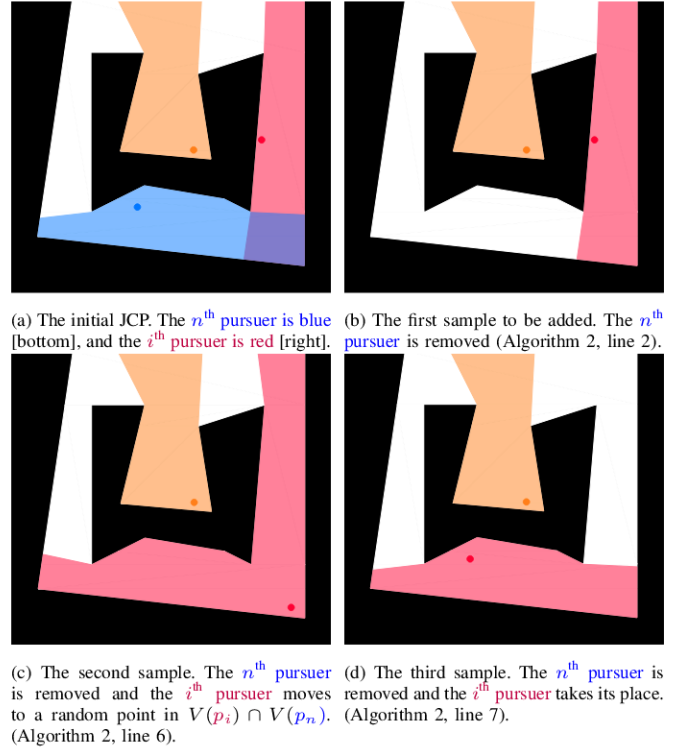
Fig. 5: An example of junction sampling.
