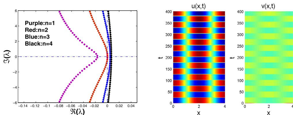
Fig. 4. The roots of (3.6) with n = 1, 2, 3, 4 (left), and periodic pattern of (3.1) (right). Here D_1 = D_2 = 1 , D_{12} = D_{21} = D_{22} = 0 , \alpha = \beta = 0.5 , \gamma = 1 , r = 25 , and D_{11} = 1.9 > 1/u^* .
