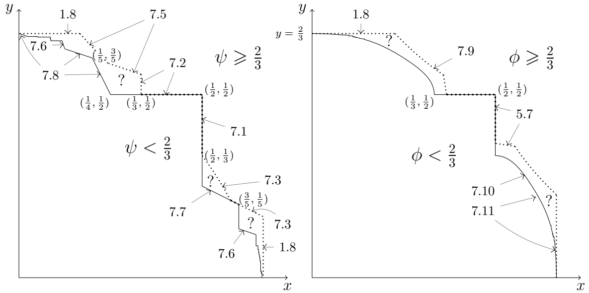
Figure 6: When \psi(x, y) < 2/3 and when \phi(x, y) < 2/3 .
