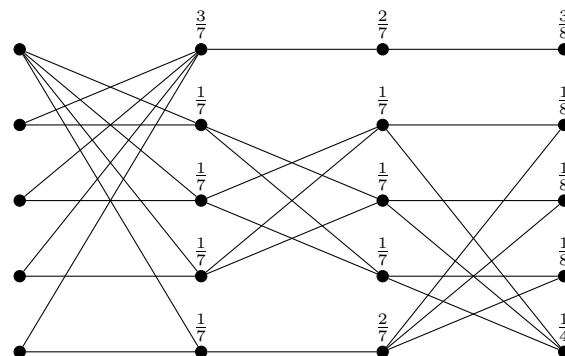
Figure 2: (4/7, 2/7, 3/8) is not triangular
