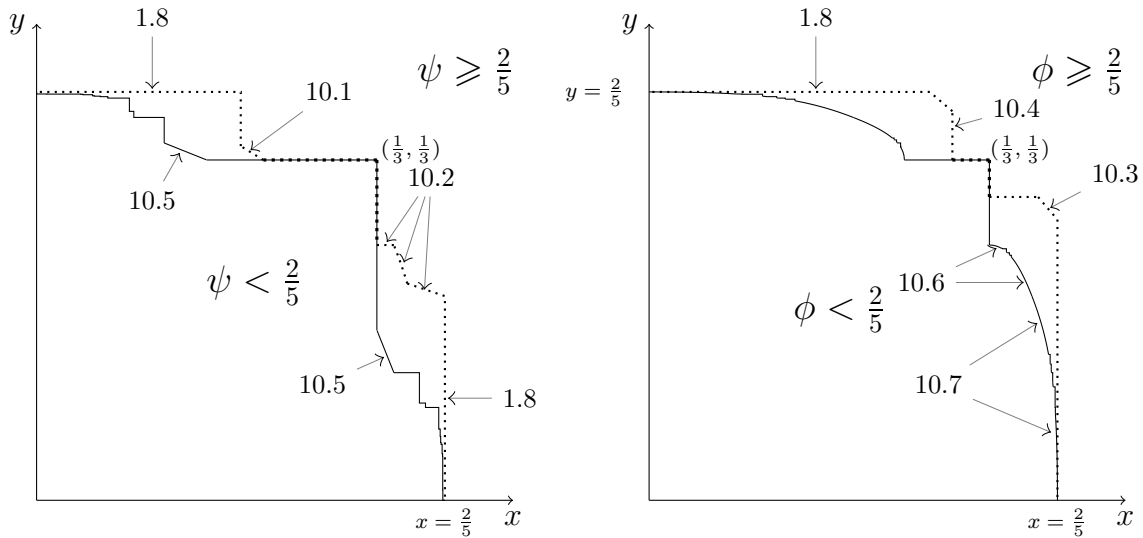
Figure 9: When \psi(x, y) < 2/5 and when \phi(x, y) < 2/5 .
