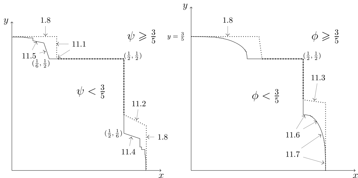
Figure 10: When \psi(x, y) < 3/5 and when \phi(x, y) < 3/5 .
