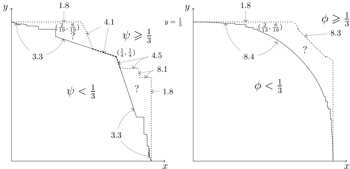
Figure 7: When \psi(x, y) < 1/3 and when \phi(x, y) < 1/3 .
