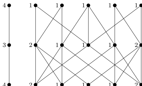
Figure 3: \phi(3/10, 4/11) \leq 4/9 .
