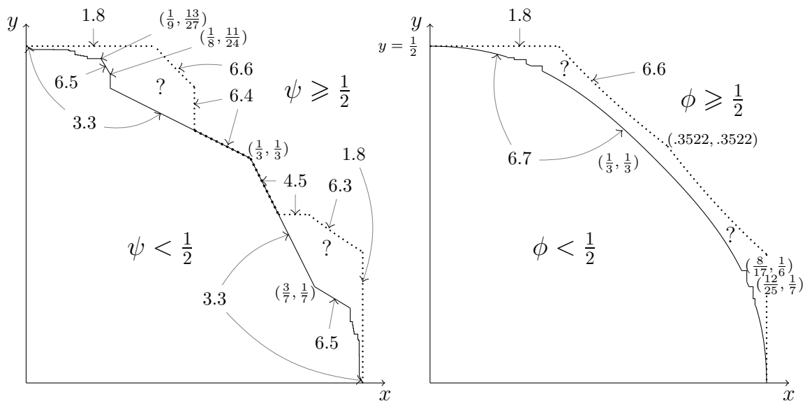
Figure 5: In the left-hand figure, \psi(x, y) < 1/2 for pairs (x, y) below the solid line, and \psi(x, y) \geq 1/2 above the dotted one; between we don't know. The right-hand figure does the same for \phi .
