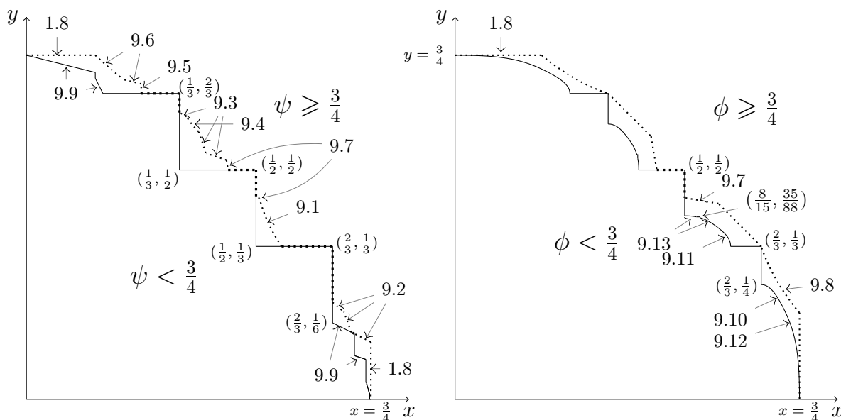
Figure 8: When \psi(x, y) < 3/4 and when \phi(x, y) < 3/4 .
