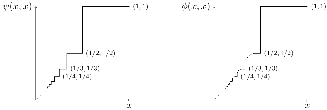
Figure 4: Graphs of \psi(x, x) and \phi(x, x)
