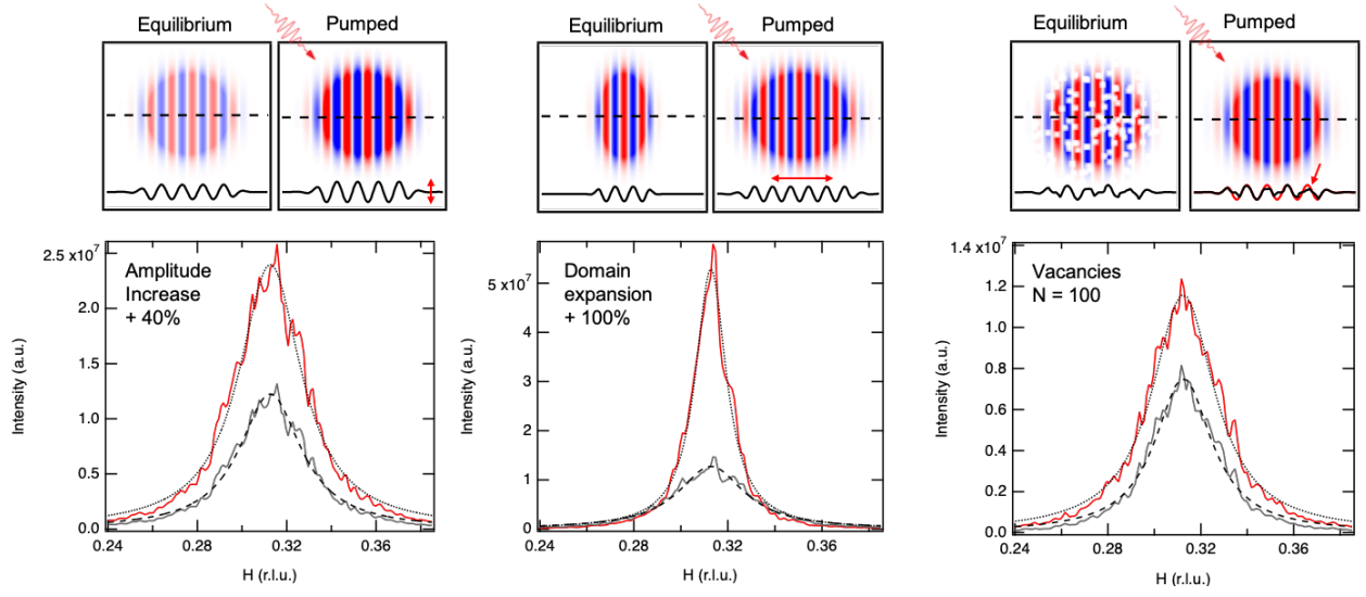
Fig. S7. Simulated x-ray scattering signal for the cases reported in Fig. 3 of the main text. A) amplitude increase, as predicted by Ginzburg-Landau theory for coexisting and homogenous orders, B) CDW domain expansion, as expected in the case of phase separation, and C) a distribution of vacancies that is removed by the laser.
