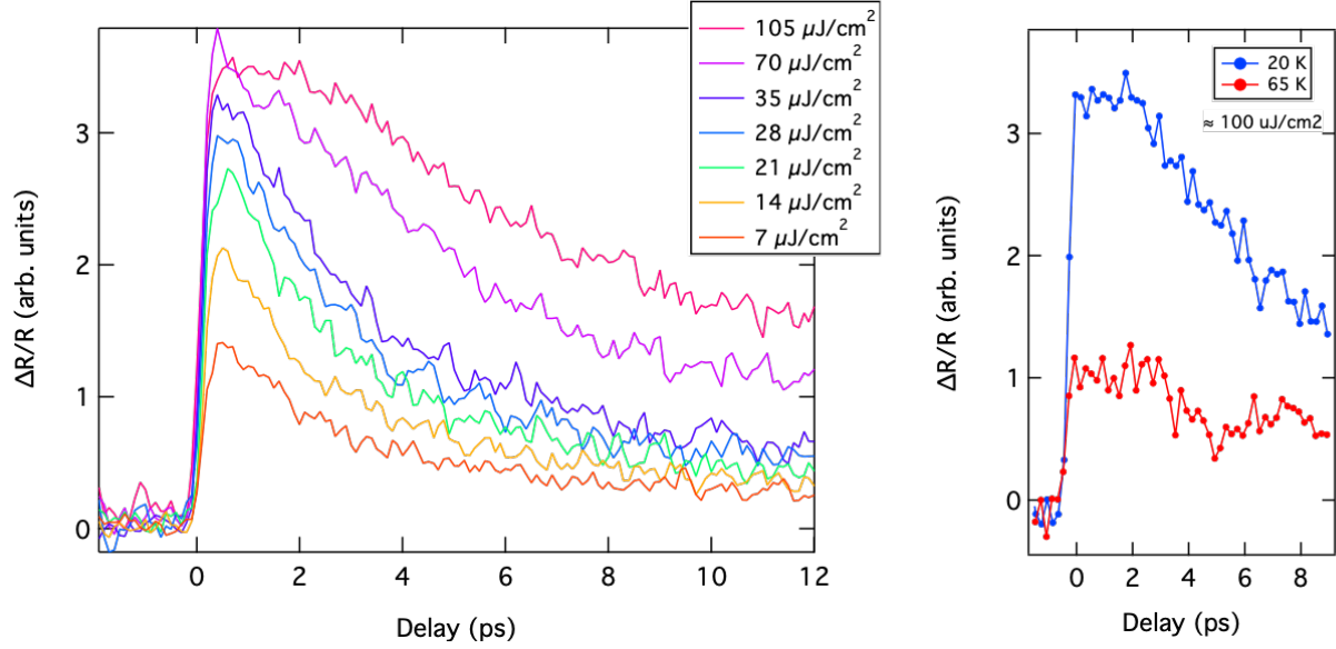
Fig. S4. A, Fluence dependence of the time-resolved reflectivity signal, 800 nm probe, in the superconducting phase of YBCO ( T = 20 K). B, Time-resolved reflectivity signal at 20 K and 65 K for \approx 100 \mu\text{J}/\text{cm}^2 . The signal drops dramatically around T_C indicating the clear connection to the SC order.
