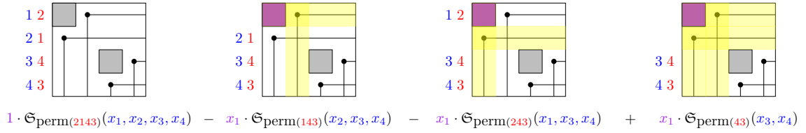
FIGURE 2. The four diagrams in this figure correspond left to right to the subwords \{v \mid u \leq v \leq w\} = \{2143, 143, 243, 43\} for w = 2143 and u = 43 as in Example 3.9. These in turn yield the Schubert polynomials in the expression (6). The red numbers on the left of the diagrams signify these subwords; the blue numbers are the row numbers yielding the variables of the corresponding Schubert polynomials in the expression (6). The purple boxes correspond to the boxes of the Rothe diagram of w = 2143 that are removed in order to obtain v ; graphically these are the boxes struck by yellow if the yellow highlighted rows and columns are extended; the row indices of these boxes yield the monomials M_{w,v} .
