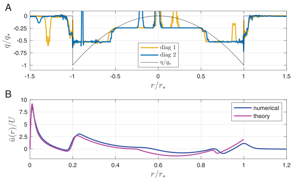
Fig. 2. (A) PV as a function of r/r_* along the diagonal cuts shown in Fig. 4A. (B) Azimuthally averaged azimuthal velocity, \bar{u}(r) as a function of r/r_* . The “numerical” curve is \bar{u}(r) calculated from the final state (8 y) of the reference run; the “theoretical” curve is \bar{u}(r) inferred from an analytic fit to the azimuthally averaged PV. The fit uses Gaussian polar cyclones embedded in a background of homogenized PV and does not attempt to model cyclonic vorticity outside the trap where r > r_* (see SI Appendix, section 6 for details).
