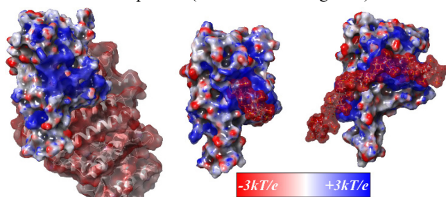
Figure 2. The 3kT/e electrostatic potential (ESP) surfaces calculated for RBD associated with ACE2 (left), fondaparinux (middle) and dp20 (right). The ACE2/RBD structure (part of PDB 6M17 28 ) shows ACE2 in a ribbon format with an ESP-mapped molecular surface. Both RBD/heparinoid complexes are representative structures from MD simulations; the heparinoids are shown in a ball-and-stick format with ESP-mapped molecular surfaces.
