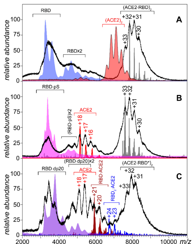
Figure 3. Mass spectra of RBD/ACE2 solutions (5 and 2.5 \mu M, respectively) in 150 mM \text{NH}_4\text{CH}_3\text{CO}_2 acquired in the absence of heparinoids (A), and in the presence of fondaparinux (B) and dp20 (C). The reference mass spectra of ACE2 is shown in panel A (red); the blue, pink and purple reference spectra in panels A, B and C, respectively, represent RBD, RBD/fondaparinux and RBD/dp20. The well-defined charge ladders in each panel show the results of limited charge reduction measurements that were used to assign the poorly-defined ion peaks in the original mass spectra.
