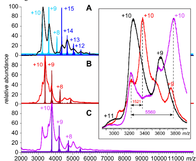
Figure 1. Mass spectra of the recombinant form of the SARS-CoV-2 S-protein RBD (10 \mu\text{M} aqueous solution in 150 mM \text{NH}_4\text{CH}_3\text{CO}_2 ) in the absence of heparinoids (A), and in the presence of 15 \mu\text{M} fondaparinux (B) and 15 \mu\text{M} fixed-length heparin oligomer dp20 (C). The charge states of the poorly-defined peaks in the original mass spectra were assigned using limited charge reduction of ionic populations at m/z 3,256 (cyan), 3,375 (maroon), 3,779 (purple) and 4,358 (blue). The inset shows a zoomed view of the ionic signals at the charge state +10 in all three mass spectra.
