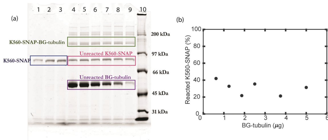
Fig. 2 Efficiency of the SNAP-based bonding reaction estimated by gel electrophoresis (a) Lanes 1–3 contain 0.87, 1.31, 1.75 μg of K560-SNAP, respectively. Lanes 4–9 contain 1.75 μg of K560-SNAP incubated with decreasing amounts of BG tubulin, 5, 3.75, 2.5, 1.87, 1.25 and 0.62 μg, respectively. Lane 10 contains the standard, SDS-broad range protein (Bio-Rad, 161-0317). The bands at 50 kDa are unreacted tubulin monomers; the bands at 84 kDa correspond to unreacted K560-SNAP, and the band at ~134 kDa correspond to linked K560-SNAP-BG-tubulin complex. All the bands at and above 200 kDa are associated with protein structures that are not fully understood. (b) Using the intensity versus amount of K560-SNAP from lane 1–3, we interpolated the amount of unreacted K560-SNAP in lanes 4–9. The difference between the total amount of K560-SNAP added in the reaction mixture and the estimated, unreacted K560-SNAP was inferred as the amount of K560-SNAP that reacted with BG-tubulin in lanes 4–9.
