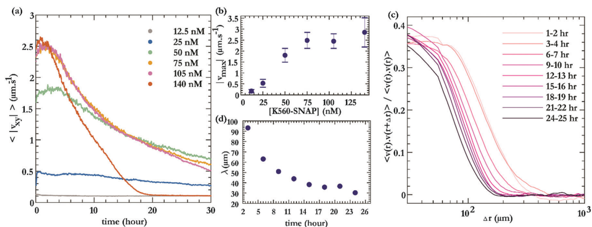
Fig. 7 Active fluid powered by K560-SNAP motors linked to BG labelled MTs. (a) Time dependence of the mean speed of tracer particles advected by the active fluid. Data is shown for different concentration of K560-SNAP. The active fluid contains only BG-MT-SNAP-K560 interactions, K560-SNAP oligomers are removed. (b) Maximum speed of tracer particles and the sample lifetime as a function of K560-SNAP concentration. (c) Time evolution of the velocity-velocity correlation of tracer particles plotted as a function of particle separation, for 50 nM K560-SNAP concentration. The spatial velocity correlation is average over one hour. (d) Time evolution of the correlation length, \lambda , extracted from the spatial correlation function. [MTs = 13.3 \mu\text{M} , ATP = 1.42 mM, pluronic = 2%, temperature = 20 ^{\circ}\text{C} ].
