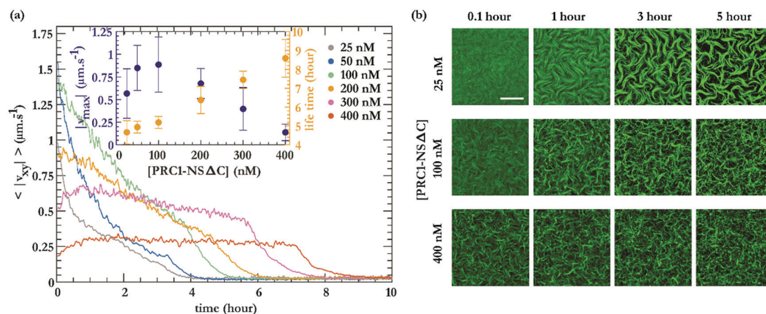
Fig. 9 Enhanced dynamics with truncated PRC1. (a) Dependence of mean speed of tracer particles on the PRC1-NSAC concentrations. Inset: Dependence of maximum speed and the fluid lifetime on PRC1-NSAC concentration. (b) Structure of active fluids consisting of different amounts of PRC1-NSAC observed with fluorescence microscopy. K401 clusters (250 nM) drive the dynamics. Images taken with fluorescence microscope. Scale bar, 500 \mu m. [MTs = 13.3 \mu M, ATP = 1.42 mM, temperature = 20 ^{\circ} C].
