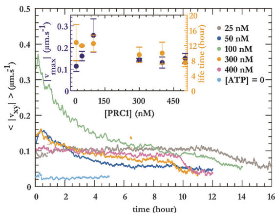
Fig. 8 Dynamics of PRC1-based active fluids. Dependence of mean speed of tracer particles on the PRC1 concentrations. Inset: Maximum speed of tracer particles and the life time of the active fluid as a function of PRC1 concentration. K401 clusters (250 nM) drive the dynamics. [MTs = 13.3 \mu M, ATP = 1.42 mM, temperature = 20 ^{\circ} C].
