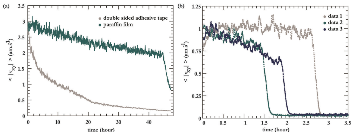
Fig. 3 Sensitivity to type of confinement and reproducibility of the active fluids. (a) Dynamics of the active fluid is sensitive to the chemical nature of the flow chamber. The flow chambers containing adhesive tape exhibit sample degradation, [BG-MTs = 13.3 \mu\text{M} , K560-SNAP = 50 nM, ATP = 1.42 mM, pluronic = 2%]. (b) Reproducibility of the active fluid dynamics with three samples that are prepared independently of each other. [MTs = 13.3 \mu\text{M} , K401-clusters = 121 nM, ATP = 1.42 mM, pluronic = 2%].
