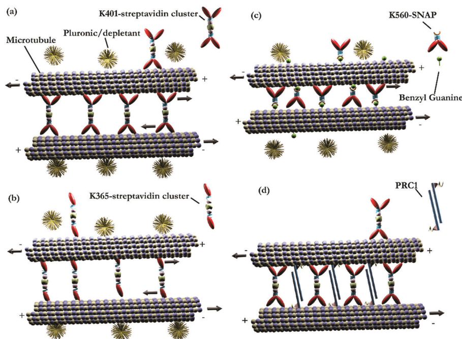
Fig. 1 Microscopic building blocks for four types of active fluids. (a) Previously studied active fluids consisted of MTs, clusters of double-headed processive kinesin motors (K401) and a depleting agent. (b) Modified active fluids powered by clusters of single-headed non-processive kinesin motors (K365). (c) Modified active fluids powered by double-headed processive kinesin K560-SNAP that is covalently bonded to the MT. (d) Modified active fluids in which non-specific depletion agent (pluronic) was replaced by PRC1, a protein that crosslinks anti-parallel MTs.
