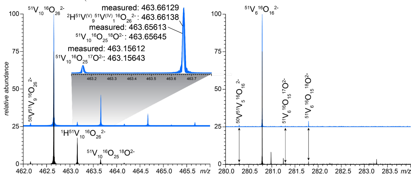
Figure 4. Zoomed views of mass spectra of V10 (sodium salt) acquired in \text{H}_2\text{O} and 2\text{H}_2\text{O} (black and blue traces, respectively) showing isotopic clusters corresponding to \text{V}_{10}\text{O}_{26}^{2-} (left) and \text{V}_6\text{O}_{16}^{2-} (right). The inset on the left panel shows the results of high-resolution measurements acquired in the narrow-band mode.
