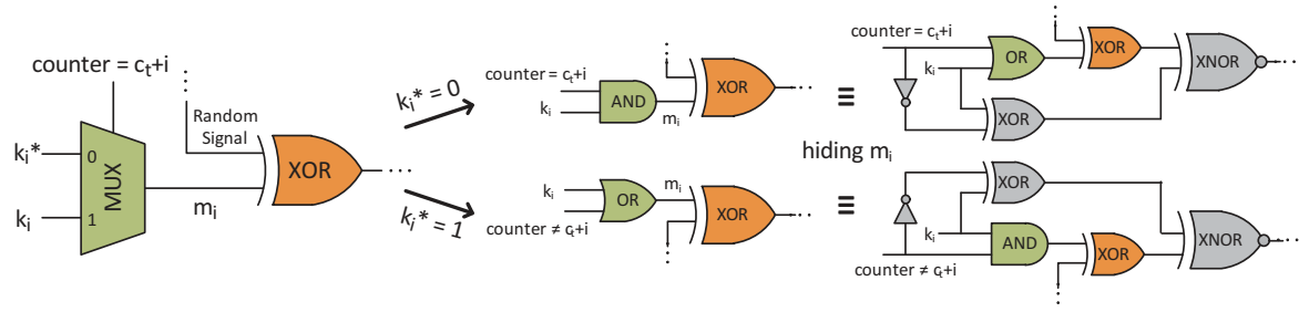
Fig. 2: A structural realization of the proposed practical encryption
