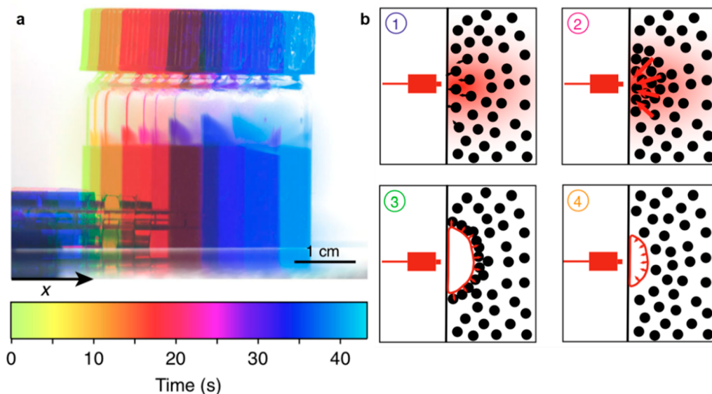
Figure 7. Optothermophoretic manipulation at the macroscopic scale. (a) Time-elased optical images showing the macroscopic motion of a vial that contains a concentrated solution of lead sulfide nanoparticles in cyclohexane. The image is a superposition of 10 snapshots of the vial position, in which different colors represent different photographing moments. (b) Schematic showing the optothermophoretic mechanism underlying the vial's motion. Adapted with permission from ref 71. Copyright 2020 Springer Nature.
