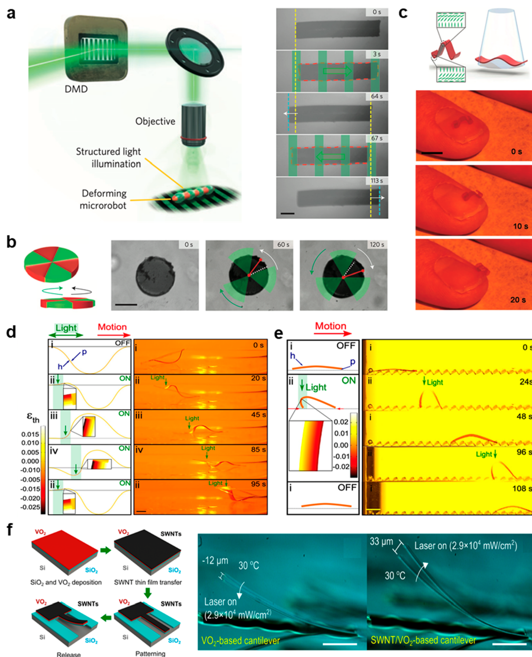
Figure 32. Optothermal actuators and robots based on phase-transition-induced shape deformation. (a) Schematic (left) and optical images (right) showing the back-and-forth crawling of an azobenzene-doped LCE microrobot under a spatiotemporally modulated laser beam. (b) Schematic (left) and optical images (right) showing the rotation of a LCE disc in an azimuthal-wave light field. Scale bars: 200 \mu\text{m} . Adapted with permission from ref 257. Copyright 2016 Springer Nature. (c) Schematic (top) and optical images (bottom) showing the walking of a LCE paper on the nail of a human finger upon temporally modulated light irradiation. Scale bar: 5 mm. Adapted with permission from ref 421. Copyright 2018 Wiley-VCH. (d, e) Schematic (with the insets showing thermal strain profiles) and optical images showing the underwater (d) crawling and (e) walking of a liquid-crystal gel paper. Scale bars: 4 mm. Adapted with permission from ref 426. Copyright 2020 National Academy of Sciences. (f) Schematic (left) showing the fabrication process and structure of CNT/VO 2 bimorph actuators driven by the optothermal phase transition of VO 2 (left) and optical images showing the amplitude difference in the optothermal oscillation of VO 2 and CNT/VO 2 bimorph actuators (right). Adapted with permission from ref 435. Copyright 2015 American Chemical Society.
