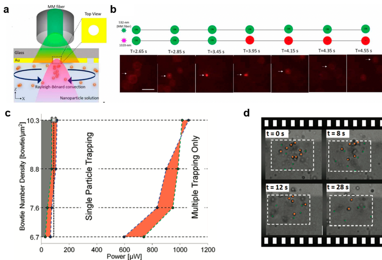
Figure 17. Optical trapping assisted by natural convection. (a) Schematic of the natural-convection-assisted plasmonic nanoaperture tweezers. (b) Optical images demonstrating the trap and release of a 200 nm fluorescent PS particle assisted by the natural convection flow. Scale bar: 25 \mu\text{m} . Adapted with permission from ref 292. Copyright 2020 American Chemical Society. (c) Hybrid phase diagram of trapping 0.5 and 1.0 \mu\text{m} PS particles on Au bowtie nanoantenna arrays. (d) Optical images showing the trapping of 0.5 \mu\text{m} PS particles and the rejection of 1.0 \mu\text{m} PS particles. The green points indicate 0.5 \mu\text{m} PS particles (trapped), and the orange points indicate 1.0 \mu\text{m} PS particles, which were repelled due to the strong thermal convection. Adapted with permission from ref 293. Copyright 2012 American Chemical Society.
