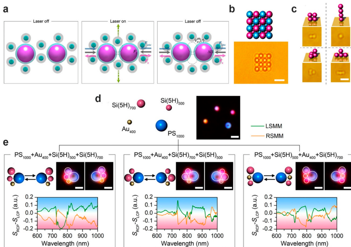
Figure 11. Opto-thermoelectric assembly of colloidal matter. (a) Schematic of the working principle of optothermal assembly. (b) 2D hybrid superlattice of silica and PS beads with various sizes. Scale bar: 5 \mu\text{m} . (c) 3D assembly of PS beads. Scale bar: 2 \mu\text{m} . Adapted with permission from ref 230. Copyright 2017 American Association for the Advancement of Science. (d) Schematic and optical images of dispersed particles as the meta-atoms to build chiral meta-molecules. (e) Schematic, optical images, and differential scattering spectra of three sets of reconfigurable chiral meta-molecules with different configurations. LSMM/RSMM indicate left-handed/right-handed meta-molecules. S_{\text{RCP}} and S_{\text{LCP}} are the scattering spectra of meta-molecules under right-handed and left-handed circularly polarized light illumination, respectively. Adapted with permission from ref 232. Copyright 2019 Elsevier.
