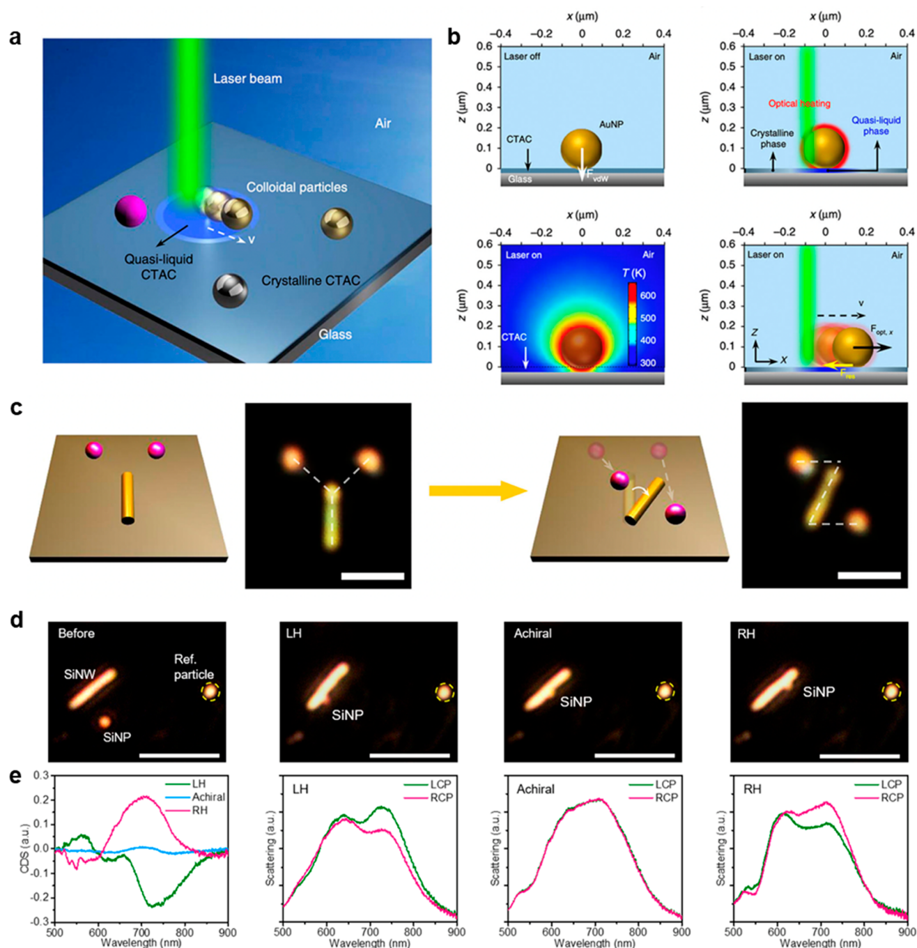
Figure 33. In-plane optical manipulation on solid substrates. (a) Schematic of OPN on a solid substrate. (b) Working principle of OPN. (c) Schematic and optical images illustrating the reconfigurable patterning of two 500 nm Si nanoparticles and one Au nanowire. Scale bar: 3 \mu m. Adapted with permission from ref 412. Copyright 2019 Springer Nature. (d) Dark-field images showing the reconfigurable assembly of left-handed (LH) structure, achiral structure, and right-handed (RH) structure in sequence from the dispersed building blocks. (e) Measured optical scattering spectra of the structures in (d) under two types of circularly polarized light (i.e., LCP, left-handed circularly polarized light; RCP, right-handed circularly polarized light) and the corresponding circular differential scattering (CDS) spectra (i.e., S_{RCP} - S_{LCP} ). Adapted with permission from ref 437. Copyright 2021 American Chemical Society.
