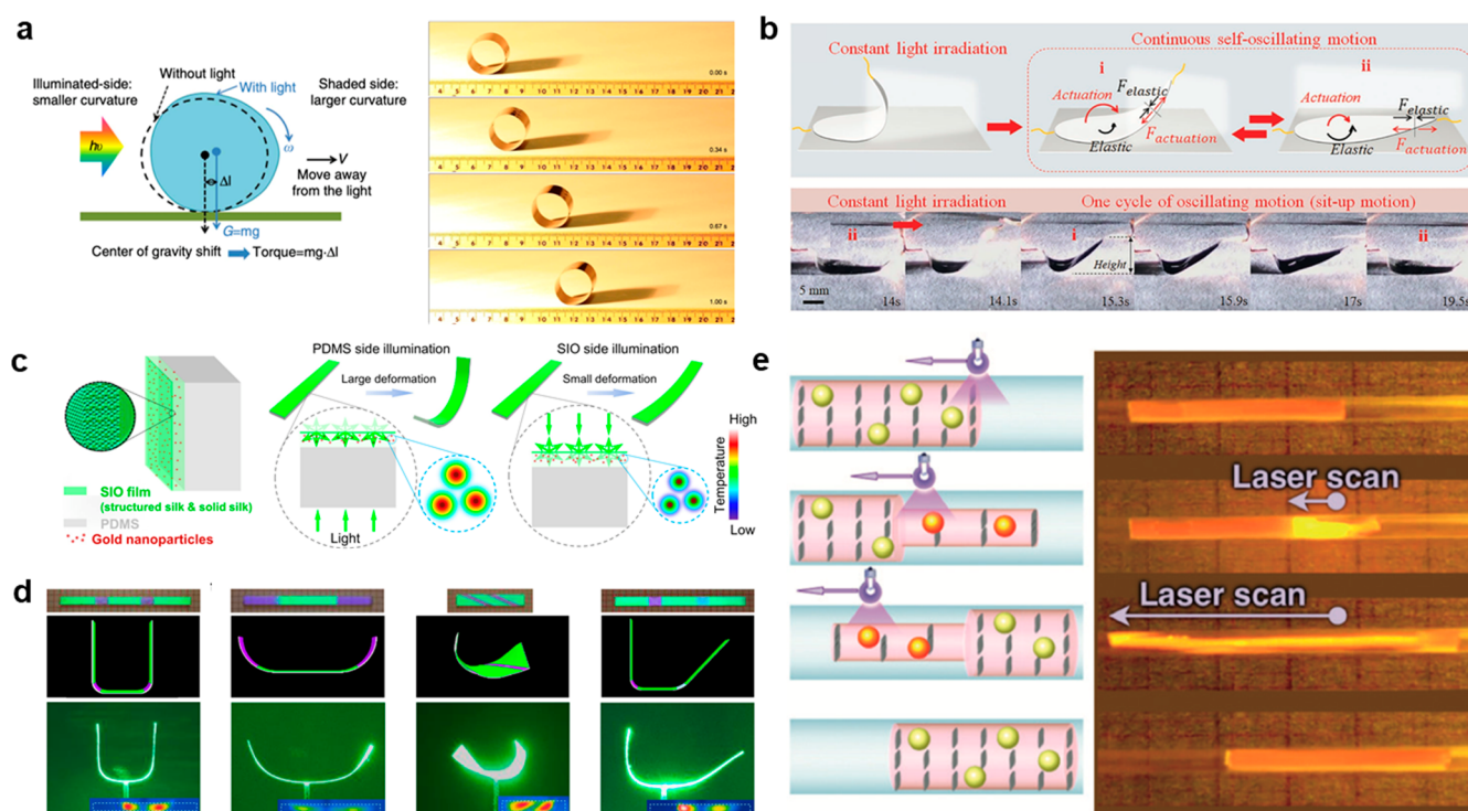
Figure 30. Optothermal actuators, motors, and robots based on thermal expansion. (a) Schematic (left) and optical images (right) showing the directional motion of a cylindrical motor upon tilted laser irradiation. Adapted with permission from ref 402. Copyright 2014 Springer Nature. (b) Schematic (top) and optical images (bottom) showing the self-sustained oscillation of a CNT/PDMS optothermal actuator via the self-shadowing effect. Adapted with permission from ref 395. Copyright 2020 Wiley-VCH. (c) Schematic showing the composition of the silk PC/PDMS bimorph structure and its tunable optothermal deformation. (d) Schematic (top) and optical images (bottom) showing the programmable deformation by patterning the silk PCs on PDMS layers. The insets are the temperature profiles at the bimorph structures upon laser irradiation. Adapted with permission from ref 80. Copyright 2021 Springer Nature. (e) Schematic (left) and optical images (right) showing the crawling of a titanate nanosheet/AuNP/PNIPAM composite in a tube upon laser scanning. Adapted with permission from ref 396. Copyright 2018 Wiley-VCH.
