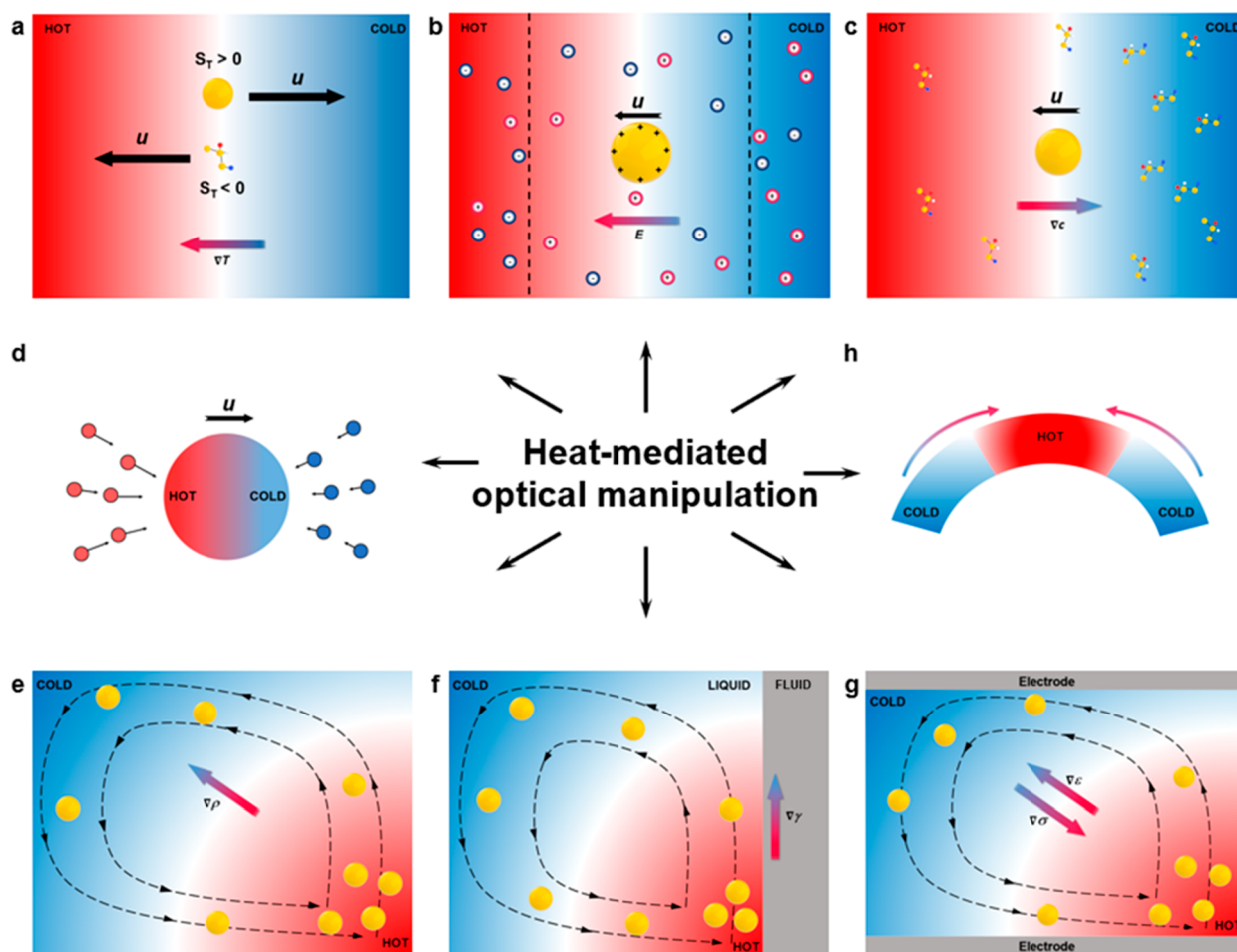
Figure 2. Schematics of physical mechanisms for heat-mediated optical manipulation: (a) thermophoresis, (b) thermoelectricity, (c) heat-mediated diffusiophoresis, (d) photophoresis ( \Delta T force), (e) natural convection, (f) heat-mediated Marangoni convection, (g) electrothermoplasmonic flow, and (h) optothermal shape deformation.
