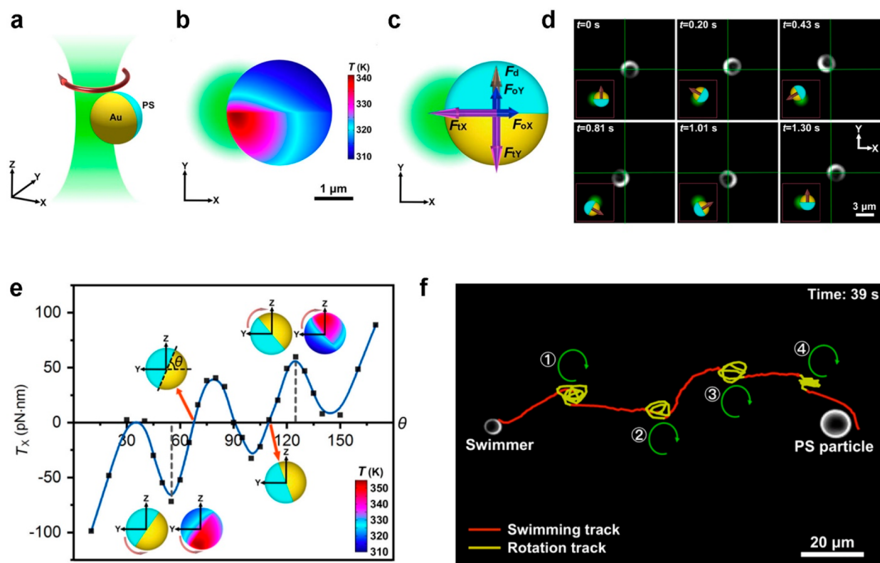
Figure 12. Opto-thermoelectric swimmers. (a) Schematic of the rotation of a PS/Au Janus particle under a focused laser beam. (b) Simulated temperature profile of the Janus particle. (c) Schematic of force analysis. (d) Time-resolved dark-field images showing the rotation of a Janus particle. (e) Calculated thermoelectric torques as a function of angle \theta , which is defined as the angle between the PS/Au interface relative to the substrate. (f) Trajectory of a Janus particle transported to a predefined target. Adapted with permission from ref 235. Copyright 2020 Springer Nature.
