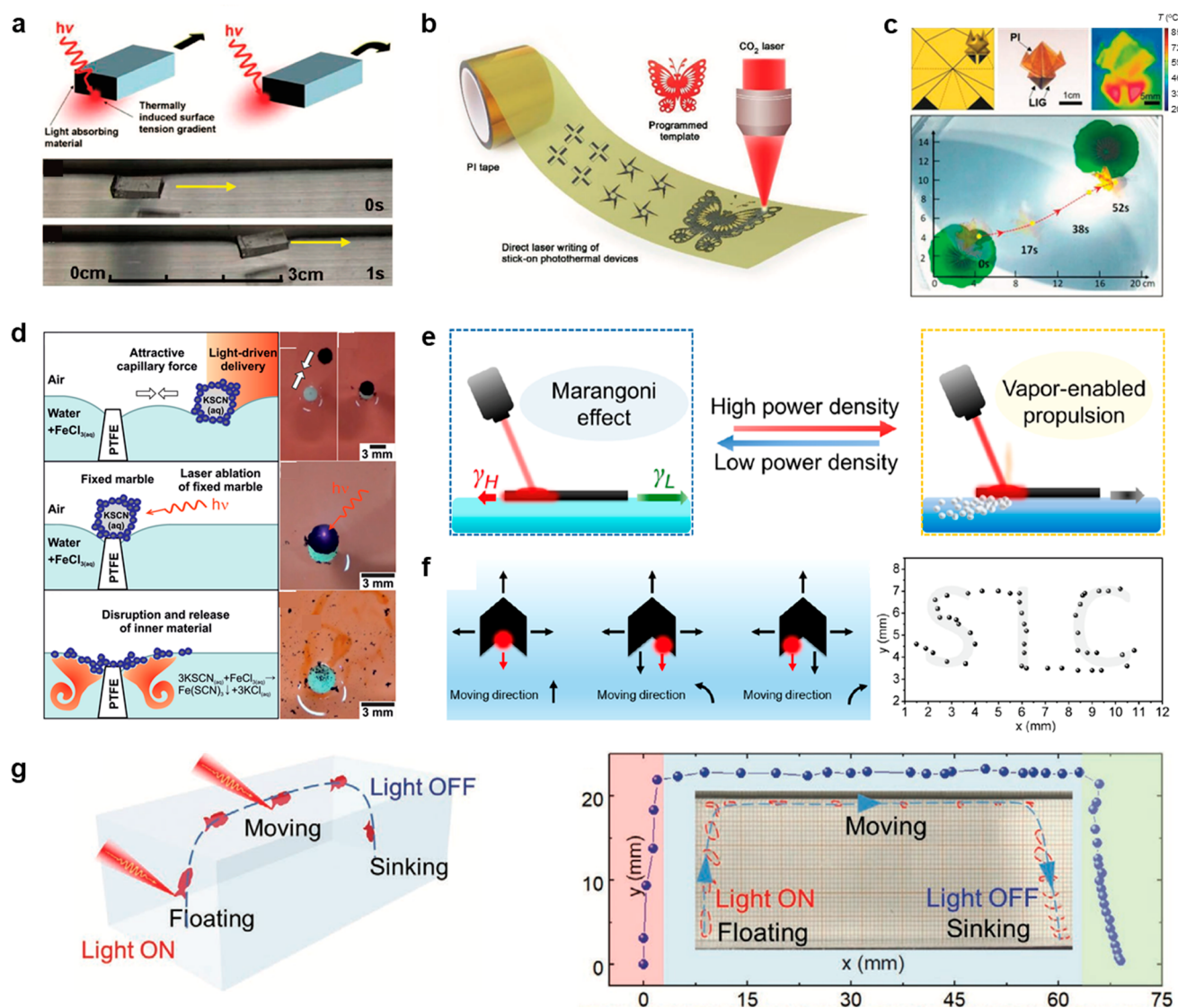
Figure 26. Optothermal Marangoni swimmers. (a) Working principle and directional motion of optothermal Marangoni swimmers composed of a PDMS block with one side coated with vertically aligned carbon nanotube forests. Adapted with permission from ref 377. Copyright 2009 American Chemical Society. (b) Schematic showing the direct laser writing on the PI tape for the fabrication of optothermal Marangoni swimmers. (c) Origami template, optical image, thermography image, and directed movement of a 3D origami froglike swimmer powered by focused sunlight. Adapted with permission from ref 382. Copyright 2021 Wiley-VCH. (d) Schematics and optical images showing fixing, and disruption/release of the liquid marble powered by NIR laser irradiation. Adapted with permission from ref 376. Copyright 2016 Wiley-VCH. (e) Schematic showing the dual-mode propulsion of the optothermal-paper-based swimmer. (f) Schematic and trajectory showing directional control of the swimmer by manipulating the laser beam position. Adapted with permission from ref 380. Copyright 2020 American Chemical Society. (g) Schematic and experimental demonstration of an optothermal swimmer with 3D motion. Adapted with permission from ref 381. Copyright 2021 Wiley-VCH.
