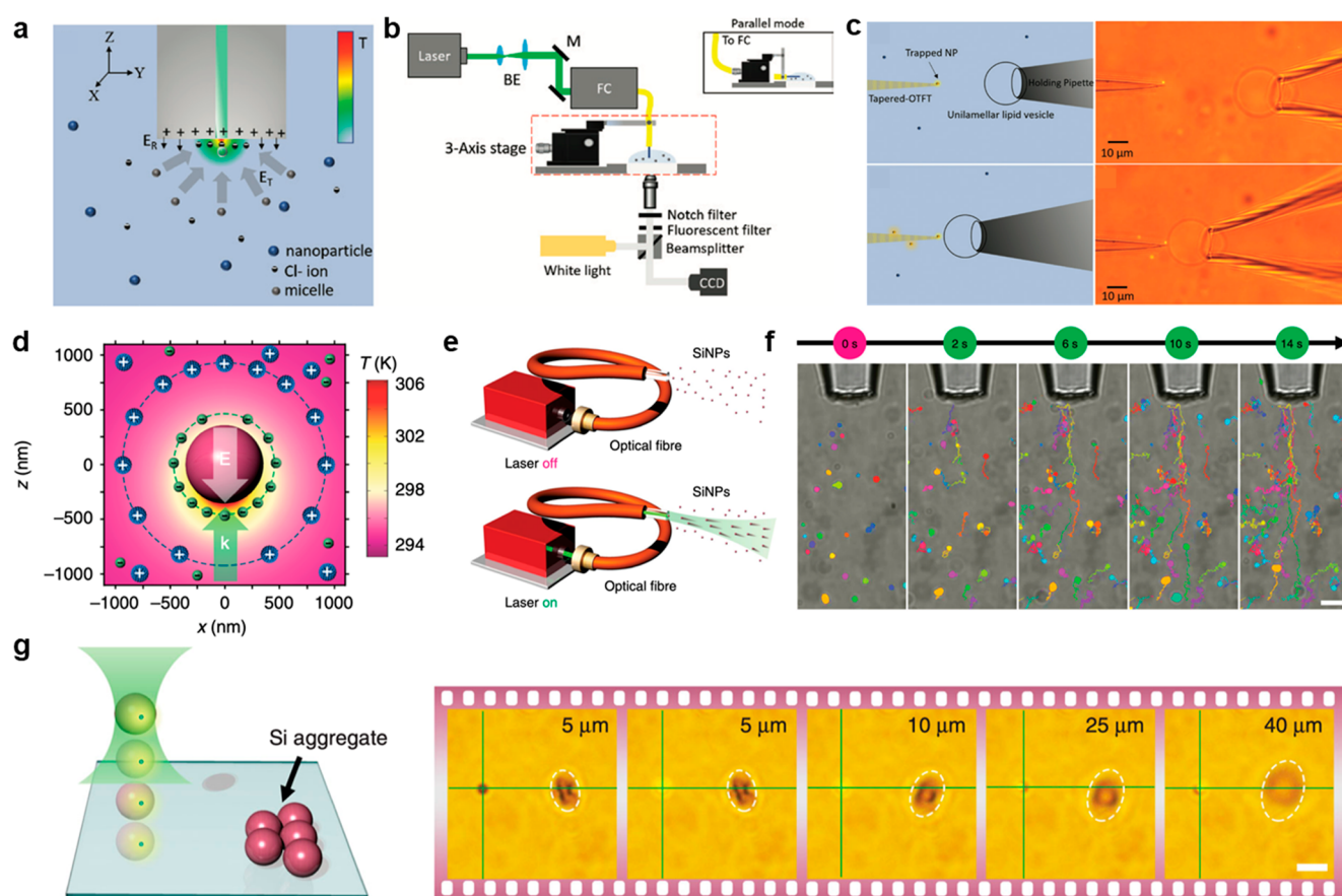
Figure 10. 3D opto-thermoelectric trapping and manipulation. (a) Schematic illustration of the working principle and (b) optical setup of opto-thermoelectric fiber tweezers (OTFT). BE, beam expander; M, mirror; FC, fiber coupler; CCD, charge-coupled device. (c) Schematics and optical images showing the single-particle delivery to a lipid vesicle. Adapted with permission from ref 229. Copyright 2019 De Gruyter. (d) Schematic of the ionic distribution, temperature field, and corresponding thermoelectric field E on a SiNP. k indicates the wave vector of the incident light. (e) Schematic of the experimental setup for opto-thermoelectric pulling. (f) Sequential optical images showing opto-thermoelectric pulling of 500 nm SiNPs. (g) Schematic and optical images showing the out-of-plane transport of a fluorescence PS bead using a single Si particle as a shuttle. Scale bar: 5 \mu\text{m} . Adapted with permission from ref 146. Copyright 2020 Springer Nature.
