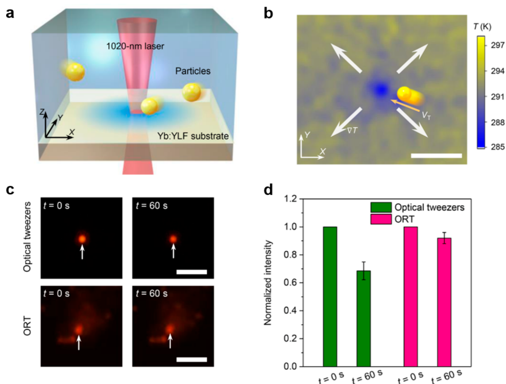
Figure 8. Opto-refrigerative tweezers. (a) Schematic of the localized laser cooling of the Yb-doped YLiF 4 substrate and the thermophoretic trapping of particles at the cold spot. (b) Measured in-plane temperature distribution at the solution–substrate interface under laser cooling with an optical intensity of 25.8 mW \mu\text{m}^{-2} . Scale bar: 10 \mu\text{m} . (c) Optical images and (d) normalized fluorescence intensity of a single 200 nm PS nanoparticle before and after being trapped by optical tweezers and ORT for 1 min. Scale bar: 5 \mu\text{m} . Adapted with permission from ref 98. Copyright 2021 American Association for the Advancement of Science.
