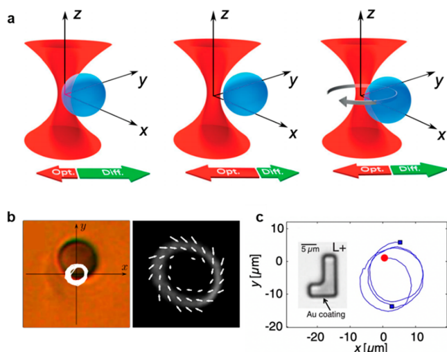
Figure 15. Optothermal diffusiophoretic rotors. (a) Schematic showing the balance between optical force (red arrows) and diffusiophoretic force (green arrows) on an optically trapped microsphere as a rotor in a critical mixture. (b) Bright-field image of the trajectories of the microsphere within 0.6 s (left) and velocity drift fields (white arrows) with particle position probability distributions (the brighter color indicates the higher probability density) (right). Adapted with permission from ref 255. Copyright 2018 American Physical Society. (c) Trajectories of an L-shaped rotor with an asymmetric gold coating. The inset is the optical image of the rotor. The red circle and blue squares indicate the initial particle position and the positions after rotation for 1 min, respectively. Adapted with permission from ref 262. Copyright 2013 American Physical Society.
