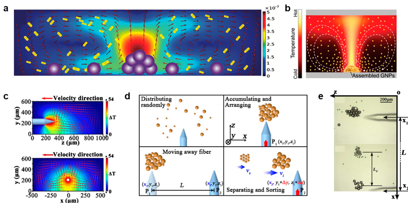
Figure 18. Optothermal assembly and sorting based on natural convection. (a) Schematic showing the natural convection flows (with a unit of \text{m s}^{-1} ) due to the light absorption of suspended Au nanorods. The convective flow concentrated hydrogel microparticles at the center of the laser spot. Adapted with permission from ref 300. Copyright 2017 Wiley-VCH. (b) Schematic showing the directed assembly and patterning of Au nanoparticles on generic substrates based on natural convection. Au nanoparticles serve as the light-absorbing medium for the optothermal generation of natural convection. Adapted with permission from ref 295. Copyright 2018 Wiley-VCH. (c) Two cross-sectional views of simulated velocity field induced by light absorption of water solution and the resultant optical heating. (d) Schematic showing the sorting process based on the thermal convection. (e) Optical images show the sorting of PS particles of different sizes. L is the displacement of the fiber tip. L_p represents the separation after the sorting. Adapted with permission from ref 72. Copyright 2016 The Optical Society.
