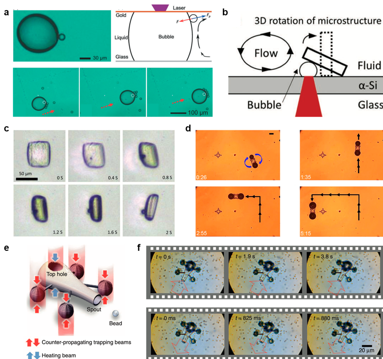
Figure 20. Optical trapping and transport based on optothermal bubbles. (a) Illustrated working mechanism and optical images of particle manipulation via optothermal bubbles. Adapted with permission from ref 318. Copyright 2014 The Royal Society of Chemistry. (b) Working principle and (c) optical images of out-of-plane rotation of microstructures based on optothermal microbubbles. Adapted with permission from ref 320. Copyright 2019 Wiley-VCH. (d) Optical images showing the manipulation of a hydrogel microstructure based on the independent movements of two microbubbles. Scale bar: 100 \mu\text{m} . Adapted with permission from ref 322. Copyright 2017 Springer Nature. (e) Schematic of a vehicle-like microstructure or microrobot. It can move with full six degrees of freedom by controlling four trapping beams (red arrows). A heating laser beam (blue arrow) propagates through the top hole to irradiate the deposited metallic layer on the hole wall for the generation of optothermal bubbles. (f) Optical images show the loading and unloading of particles based on optothermally controlled Marangoni convection at the bubbles inside the hole of the robot. Adapted with permission from ref 324. Copyright 2016 Springer Nature.
