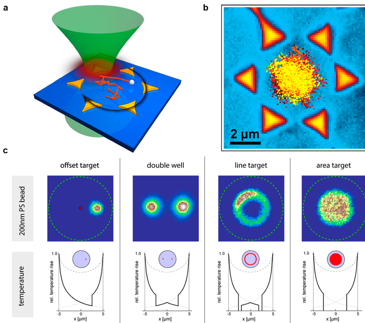
Figure 5. Optothermophoretic trapping of thermophobic objects. (a) Schematic and (b) trajectory points showing the thermophoretic trapping of a 200 nm PS bead under a rotating laser beam. Adapted with permission from ref 208. Copyright 2013 American Chemical Society. (c) Different trapping modes based on different feedback-control rules of the heating laser. The top row represents the probability density distribution of trapped particles, and the bottom one shows the corresponding temperature rise. Adapted with permission from ref 210. Copyright 2015 American Chemical Society.
