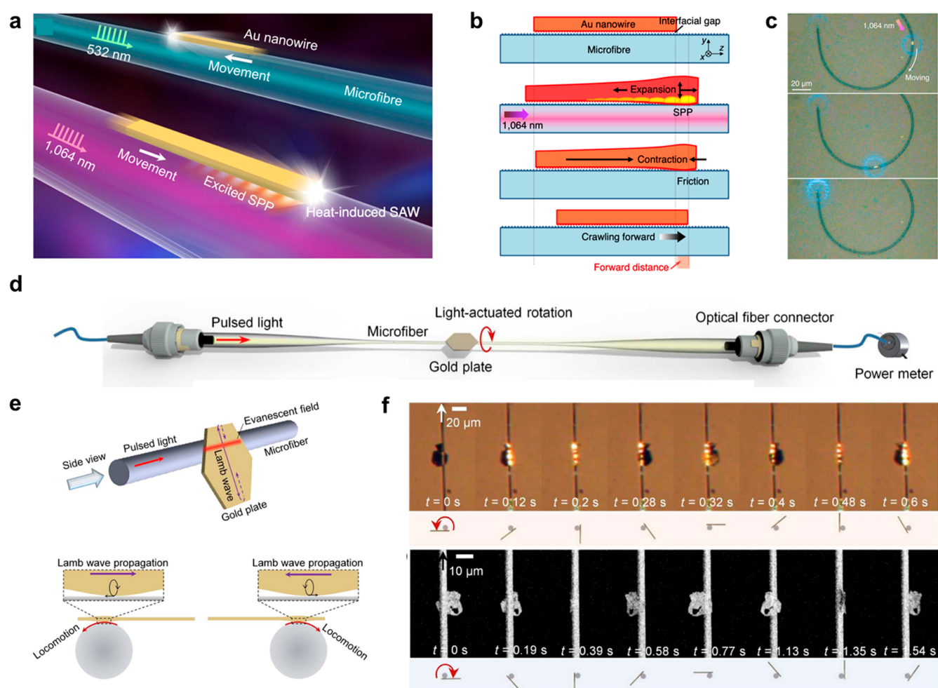
Figure 35. Crawling and rotation of metal nanostructures driven by optothermally induced surface acoustic waves in nonliquid environments. (a) Schematic showing the crawling of Au nanowires on a microfiber powered by a pulsed laser with different wavelengths. SPP, surface plasmon polaritons. (b) Working mechanism of the Au nanowire's crawling. (c) Optical images showing the movement of a Au nanowire on a C-shaped fiber. Adapted with permission from ref 168. Copyright 2021 Springer Nature. (d) Schematic showing light-actuated rotation of a Au nanoplate around a microfiber. (e) Working mechanism of the Au nanoplate's rotation. The Lamb wave is one type of SAW generated when the thickness of the nanoplate is smaller than the wavelength of the incident light. (f) Optical images and scanning electron micrographs showing the clockwise and anticlockwise rotation of a Au nanoplate around a microfiber. Adapted with permission from ref 454. Copyright 2019 American Association for the Advancement of Science.
