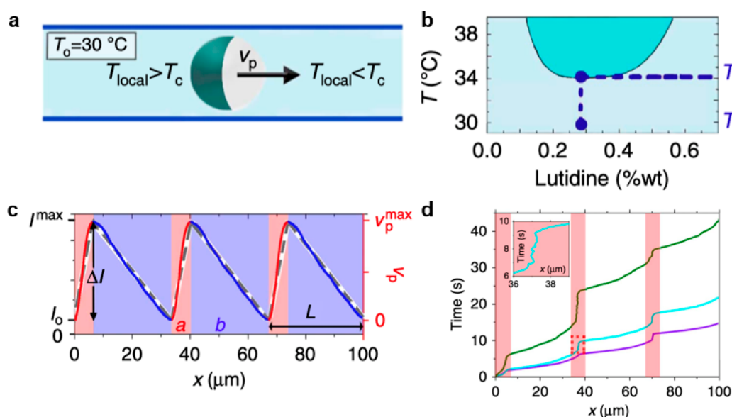
Figure 14. Optothermal diffusiophoretic microswimmers in binary critical mixtures. (a) Schematic of the working mechanism of optothermal diffusiophoretic microswimmers. (b) Phase diagram of the binary critical mixture of water–2,6-lutidine. The dark-colored region indicates the demixing region of binary mixtures. (c) Experimental (solid line) and numerical (dashed line) intensity profiles. a and b represent the lengths of positive and negative \nabla I , respectively. v_p represents the velocity of the illuminated particle. (j) Particle trajectories under different \nabla I . The inset shows the back-and-forth motion of a particle of the framed region. Adapted with permission from ref 181. Copyright 2016 Springer Nature.
