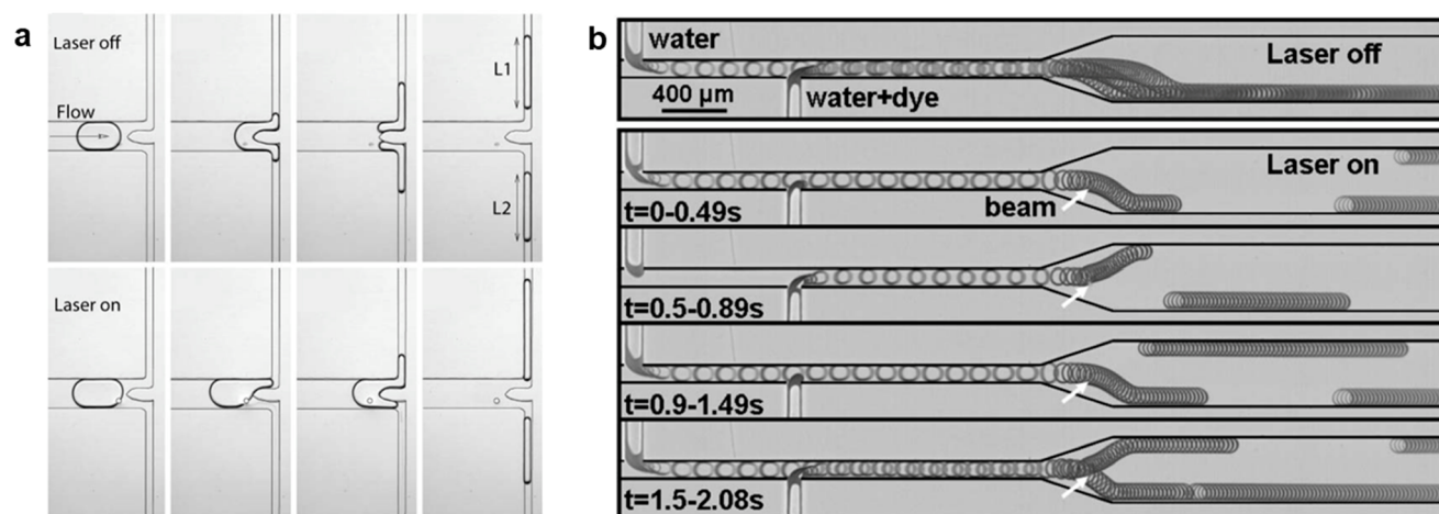
Figure 24. Optical manipulation of droplets based on Marangoni convection. (a) Optical images showing how Marangoni convection controls the division of droplets. With the heating laser off, the droplet was divided evenly into two daughter droplets (top). With the heating laser on, two uneven daughter droplets were generated (bottom). Adapted with permission from ref 367. Copyright 2007 The Royal Society of Chemistry. (b) Sorting of pure water and water–dye droplets based on optothermally induced Marangoni effect at the droplets. Each of the images was obtained by superimposing ~200 frames of individual images. Adapted with permission from ref 369. Copyright 2008 American Institute of Physics.
