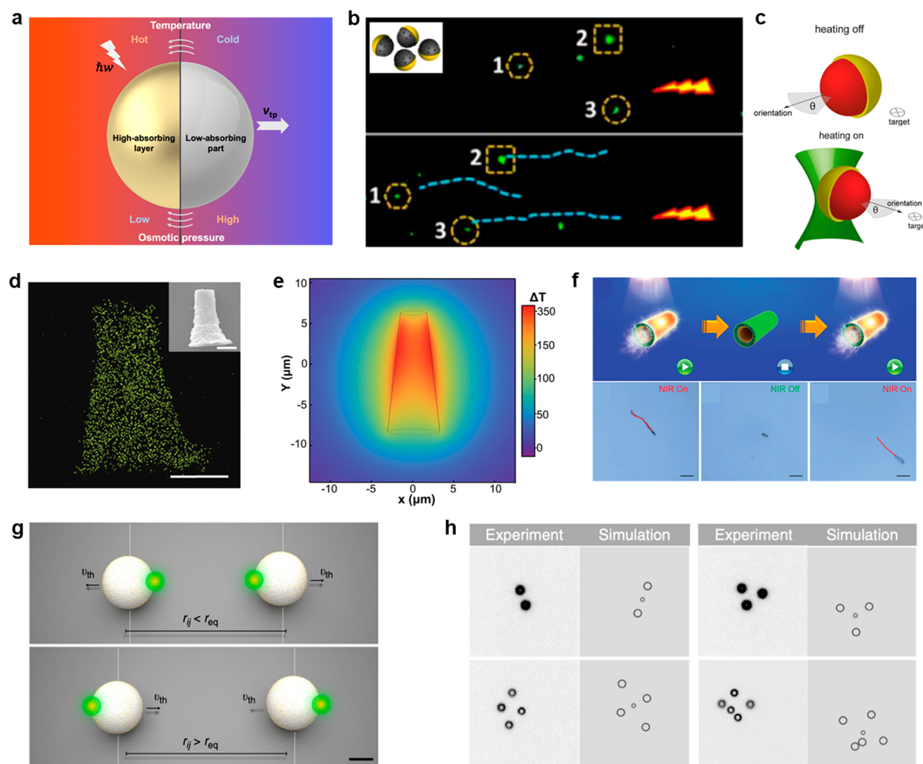
Figure 3. Optothermophoretic swimmers. (a) Schematic showing the working mechanism of optothermophoretic swimmers based on self-thermophoresis. v_{tp} is the thermophoretic velocity of the swimmer. (b) Time-revolved optical images of 80 nm Janus swimmers triggered by the NIR laser. The inset shows the schematic of the Janus swimmers. Adapted with permission from ref 184. Copyright 2016 American Chemical Society. (c) Schematic showing the working principle of directional control of self-thermophoretic swimmers. \theta is the acceptance angle for directional target delivery. Adapted with permission from ref 179. Copyright 2014 American Chemical Society. (d) Energy-dispersive X-ray spectroscopy (EDX) mapping of the tubular rocket with Au nanoshells. The inset shows the corresponding scanning electron micrograph. Scale bars: 2 \mu\text{m} . (e) Simulated steady-state temperature distribution of the rocket under laser illumination. (f) Schematic (top) and time-lapsed optical images showing the thermophoretic motions of the rocket. Scale bars: 20 \mu\text{m} . Adapted with permission from ref 180. Copyright 2016 Wiley-VCH. (g) Schematic of the pair interaction rule used to keep active particles (i.e., swimmers) at a constant interparticle distance. r_{ij} and r_{eq} represent the real-time distance and prescribed separation distance between two particles, respectively. Scale bar: 7 \mu\text{m} . (h) Simulations and experimental demonstrations of different structures arising from the interacting active particles based on the pair interaction rule. Adapted with permission from ref 10. Copyright 2018 Springer Nature.
