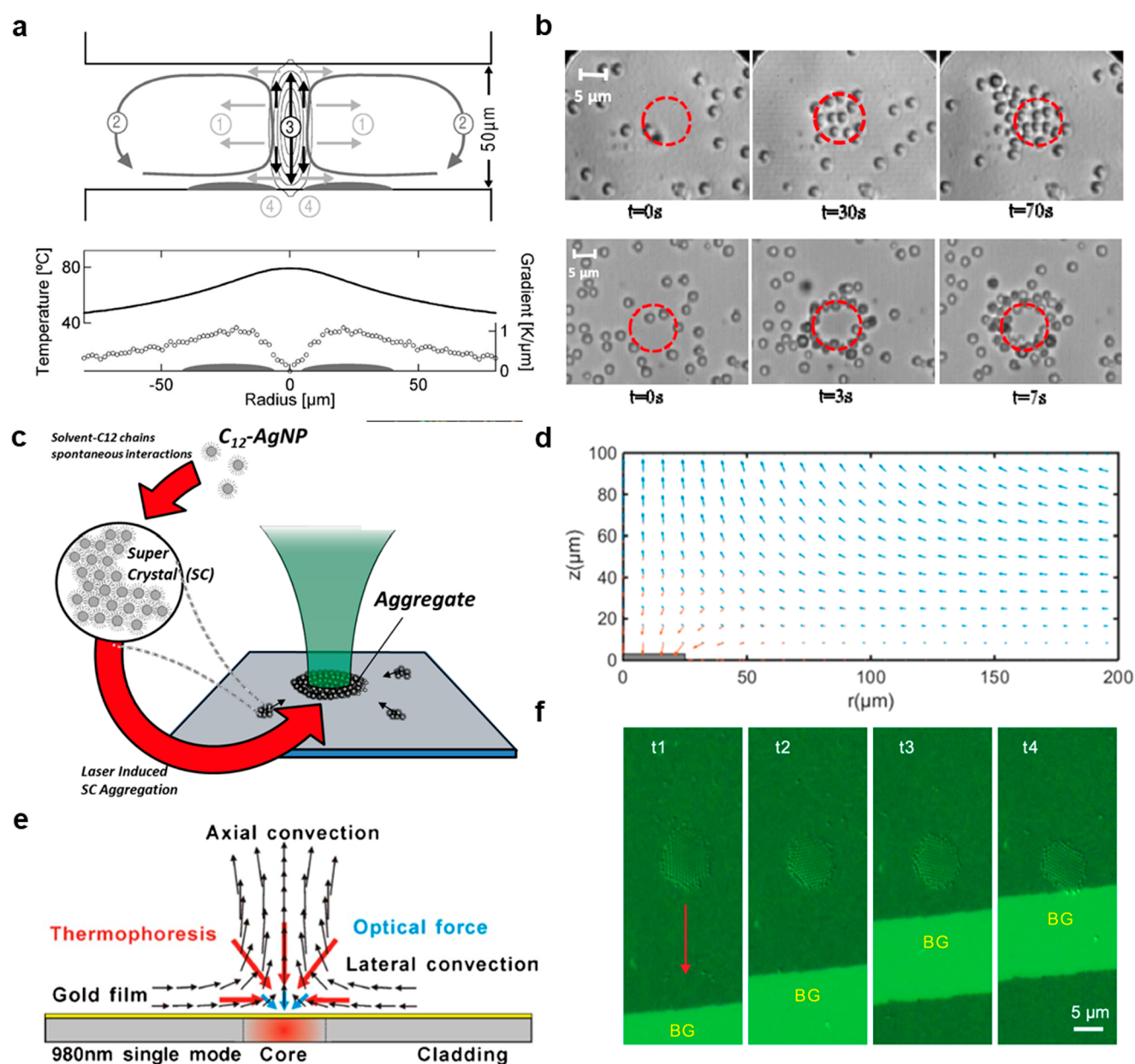
Figure 19. Optical manipulation based on natural convection combined with thermophoresis. (a) Schematic showing the formation of ring-shaped particle assemblies based on the interplay of thermophoresis and natural convection. Adapted with permission from ref 302. Copyright 2002 American Physical Society. (b) Particle accumulation around the laser spot at an incident power of 0.8 mW (top) and 6 mW (bottom). Adapted with permission from ref 68. Copyright 2015 The Optical Society. (c) Schematic showing the formation of supercrystals based on negative thermophoresis and natural convection. (d) Simulated velocity field around the aggregation. Blue and red arrows correspond to the contribution of natural convection and thermophoresis, respectively. Adapted with permission from ref 288. Copyright 2018 American Chemical Society. (e) Schematic showing the long-range trapping mechanism based on natural convection, negative thermophoresis, and optical force. Adapted with permission from ref 307. Copyright 2015 The Optical Society. (f) Optical images showing the manipulation of assembled PS particles by moving the laser spot. BG, bare glass. Adapted with permission from ref 77. Copyright 2015 Springer Nature.
