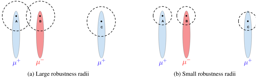
Figure 1: A data distribution demonstrating the difficulties with fixed radius balls for robustness regions. The red represents negatively labeled points, and the blue positive. If the robustness radius is set too large (panel (a)), then the regions of A and B intersect leading to a loss of accuracy. If the radius is set too small (panel (b)), this leads to a loss of robustness at point C where in principle it should be possible to defend against a larger amount of adversarial attacks.
