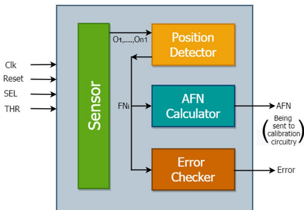
Fig. 11 Hardware implementation of sensor peripherals
