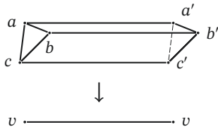
Figure 2. There are six isomorphism classes of families of (equilateral, side-length-1) triangles over a circle.
