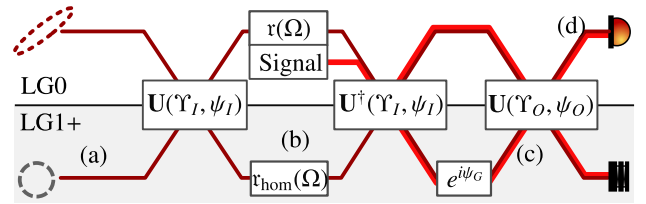
FIG. 5. Propagation of the squeezed beam and unsqueezed higher-order transverse beam modes from source to readout. The stages (a)–(d) correspond to the components in Fig. 1, depicting the matrix math of Eqs. (73)–(76). \Upsilon_I represents the transverse mismatch loss of the squeezing to interferometer, and \Upsilon_O is the mismatch of the squeezing to readout via the output mode cleaner (OMC). These mismatches cause beam-splitter-like mixing between the LG0 and LG1+ modes through Eq. (72). \psi_I, \psi_O, \psi_G are unmeasured phasing terms of the interferometer and output mismatch and of the Gouy-phase advance from the beam propagating to the output mode cleaner.
