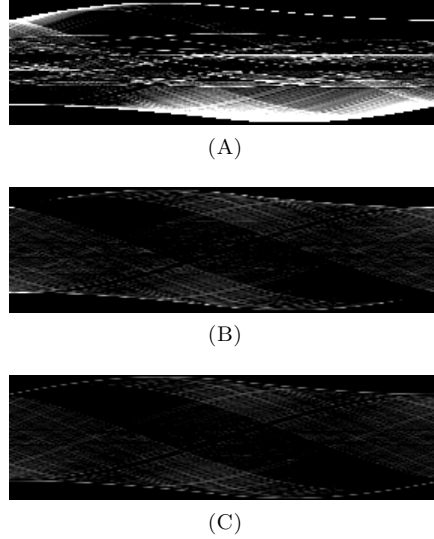
FIGURE 3. The residual sinograms of the three models: (A) Conventional discrete model; (B) Integral equation model with the piecewise constant basis; (C) Integral equation model with the piecewise linear basis for NEMA-IEC.
