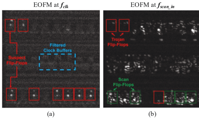
Figure 5. Processed EOFM images of the Trust-Hub Trojan benchmark with: (a) Suspect flip-flop identification. (b) Trojan flip-flop detection [48].
