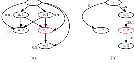
Fig. 3: (a) A time-expanded network G_S with terminal set S = \{(v,2)\} (shown in red) and node weights is shown. To obtain edge weights assume that \beta = \gamma = 1 and W_e((u,1), (v,2)) = W_e((v,1), (u,2)) = 1 . Suppose we want to solve DIRECTED PCST with \alpha = 10 . (b) After reducing DIRECTED PCST to DST, we get a graph G' with modified edge weights and no node weights. An optimal directed Steiner tree T on graph G' is shown on the right; W_{DST}(T, G') = 3 \times (-8) + 28.1 = 4.1 . Also note that W_{PCST}(T, G_S) = 4 \times 1 + 10 \times 0.01 = 4.1 , showing that W_{DST}(T, G') = W_{PCST}(T, G_S) . Note that since edge weights can be negative, leaves of an optimal directed Steiner tree need not be terminals.
