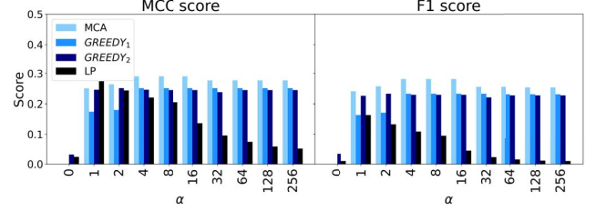
Fig. 5: The effect of varying \alpha on the performance measured by MCC (left) and F_1 -score (right). We see a sharp increase of the performance from \alpha = 0 to \alpha = 1 , followed by a minor increase, then a gradual decrease as \alpha increases.
