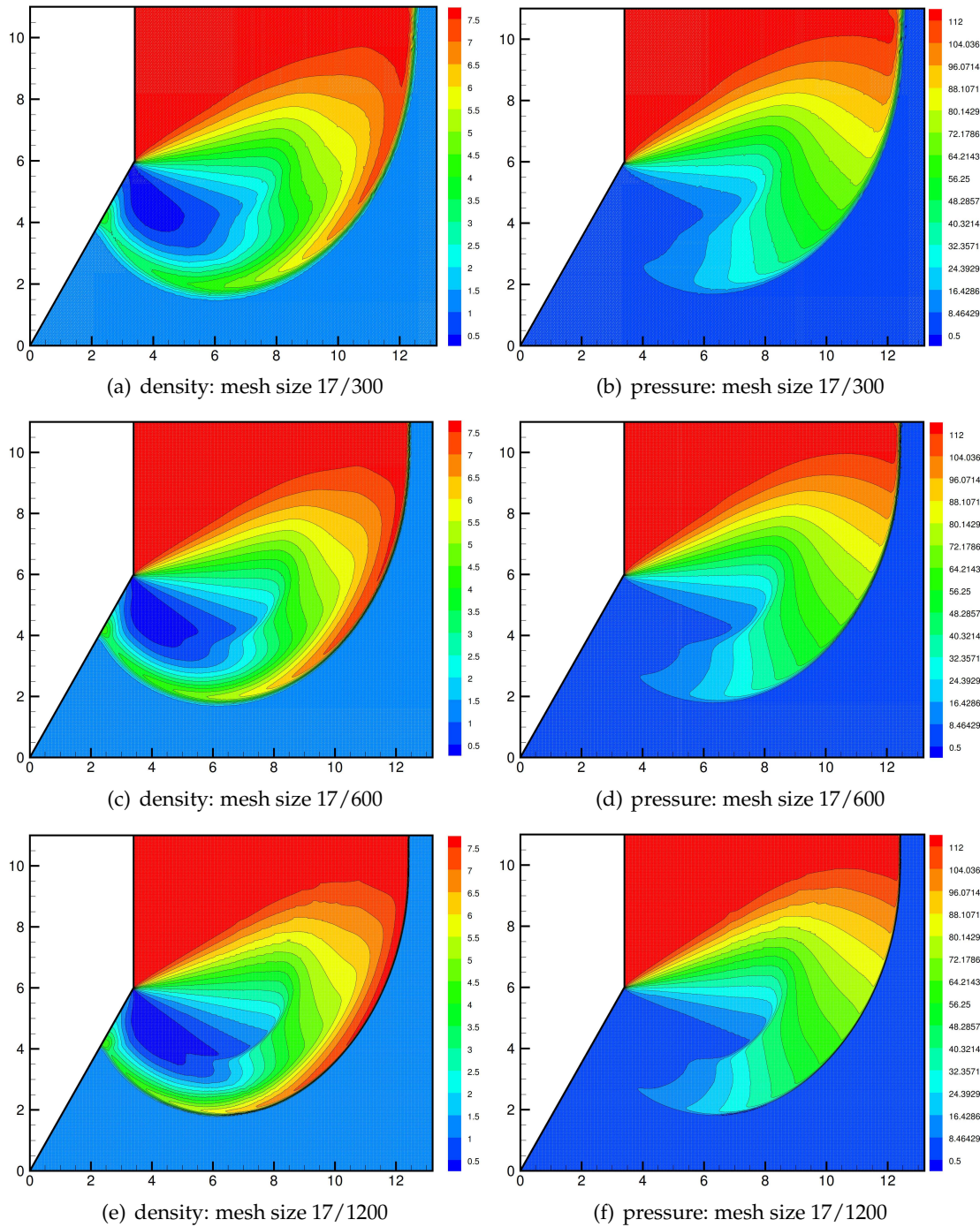
Figure 11: Example 5.12, 15 uniform contour plots of density from 0.5 to 7.5 and pressure from 0.5 to 112 at time T=0.9 .
