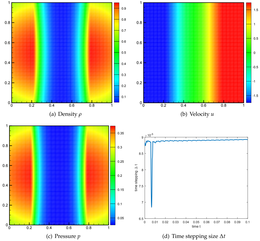
Figure 8: Example 5.10, numerical solutions by 12800 triangular meshes at T=0.1 .
