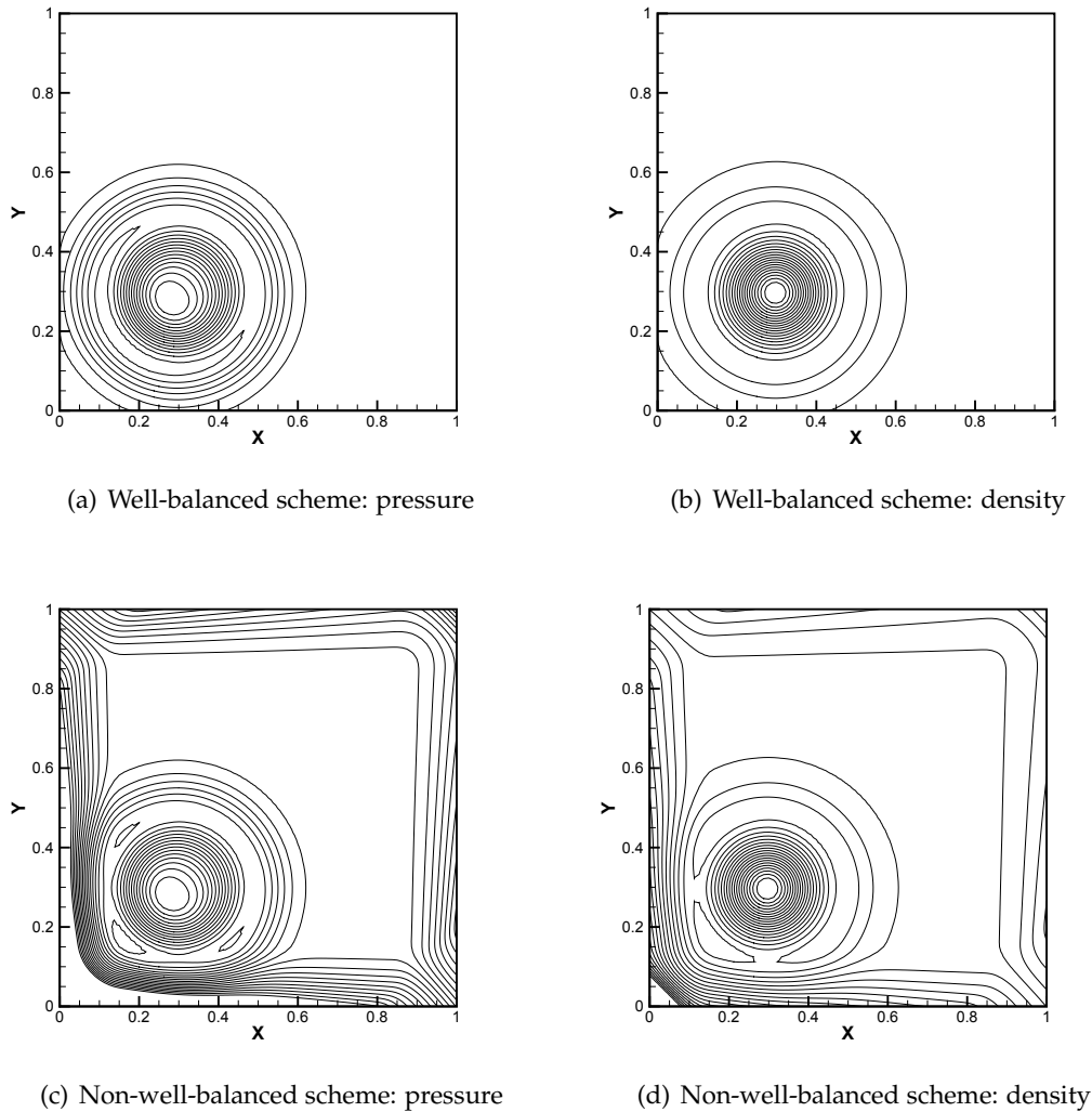
Figure 7: Example 5.9, perturbation on the isothermal hydrostatic solution with \epsilon=0.001 at time t=0.15 . Left: the pressure perturbation with 20 uniformly spaced contour lines from -0.0003 to 0.0003 ; Right: the density perturbation with 20 uniformly spaced contour lines from -0.001 to 0.0002 .
