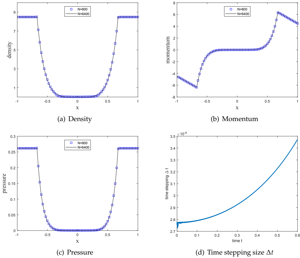
Figure 4: Example 5.6, numerical solutions at T=0.6 with 800 cells (blue squares) and 6400 cells (black solid lines). Bottom right is the figure of time stepping size \Delta t versus time t \in [0, 0.6] .
