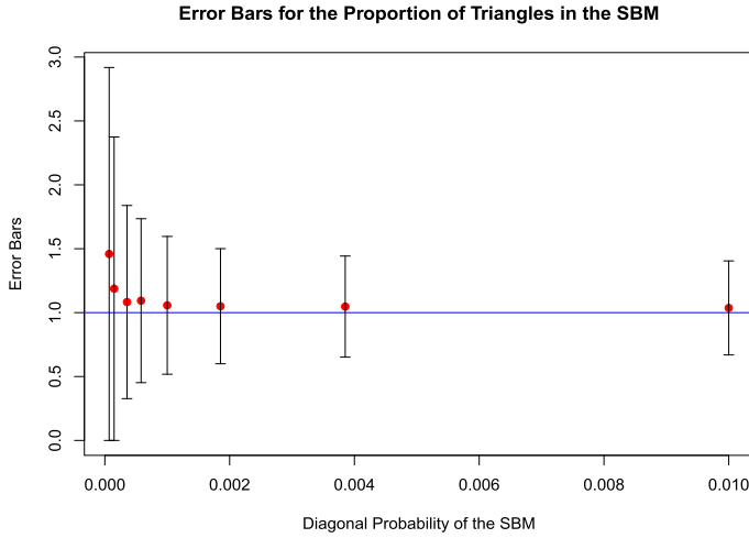
FIG. 2. Error bars for \hat{N}(K_3, G_n)/N(K_3, G_n) in a 2-block stochastic block model on n = 10,000 vertices and equal block size, with off-diagonal probability 0.5 and diagonal probability varying between 0 and 0.01 (shown along the horizontal axis).
